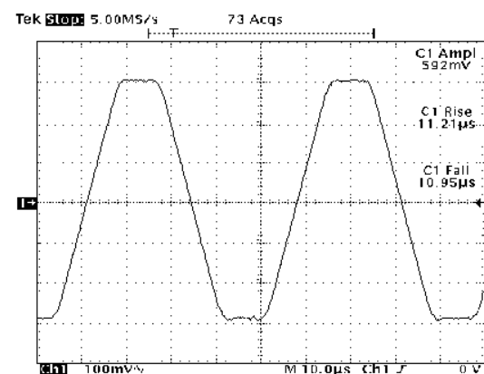
Figure 18 : 22KHz Tone
