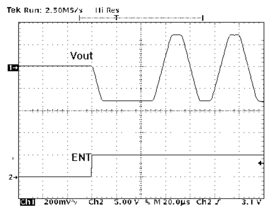
Figure 16 : Tone Enable
