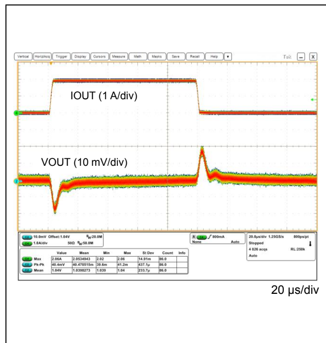
Figure 75. VOUT4 Load Transient (IOUT = 0 A to 2.05 A (SR = 1 A/ \mu s))
