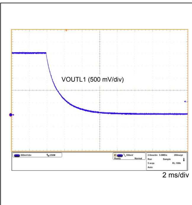
Figure 69. VOUTL1 Power OFF Waveform
