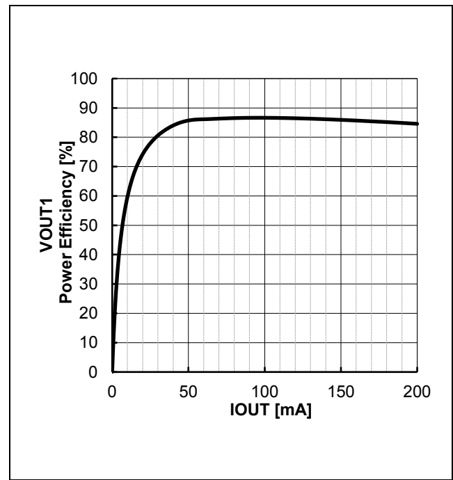
Figure 52. VOUT1 Power Efficiency vs IOU
