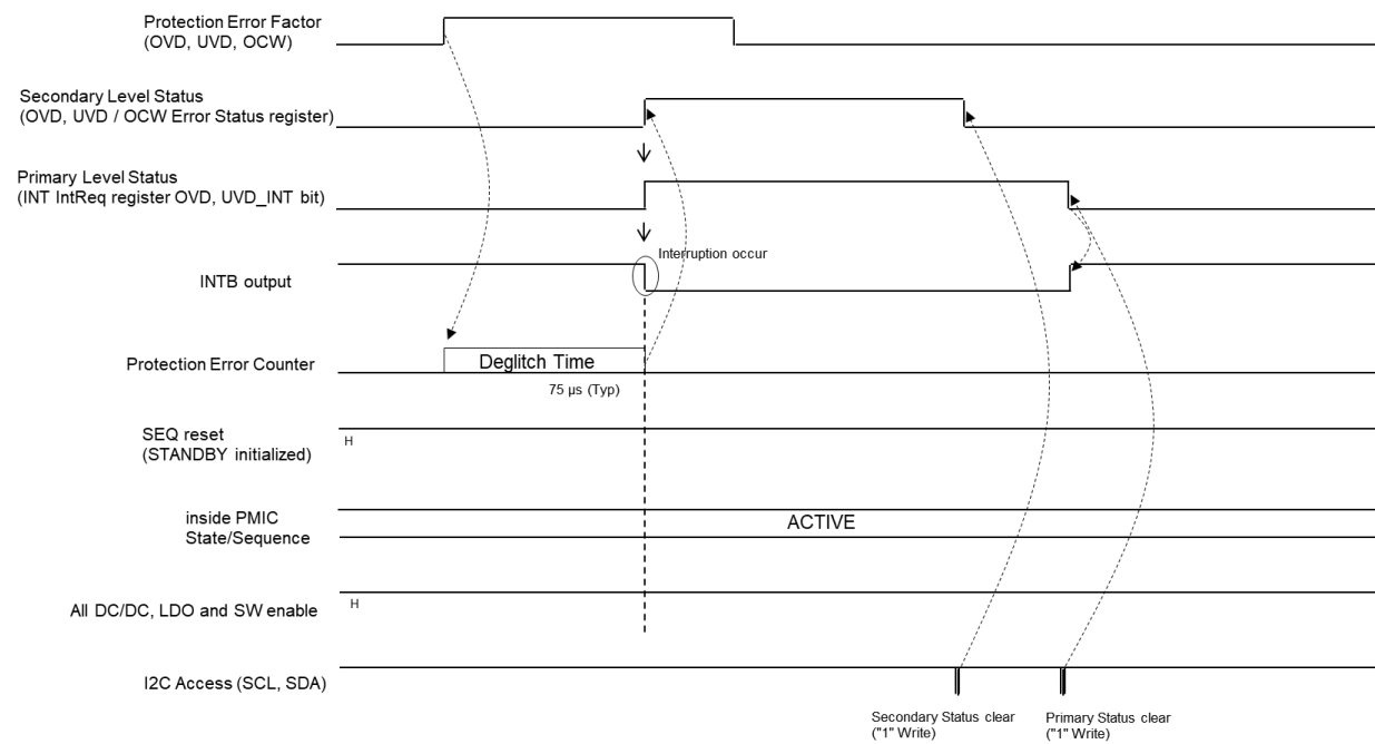
Figure 34. Timing Chart when Protection Detection Factor Occur
