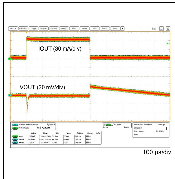
Figure 76. VOUTL1 Load Transient (IOUT = 0 A to 75 mA (SR = 100 mA/ \mu s))
