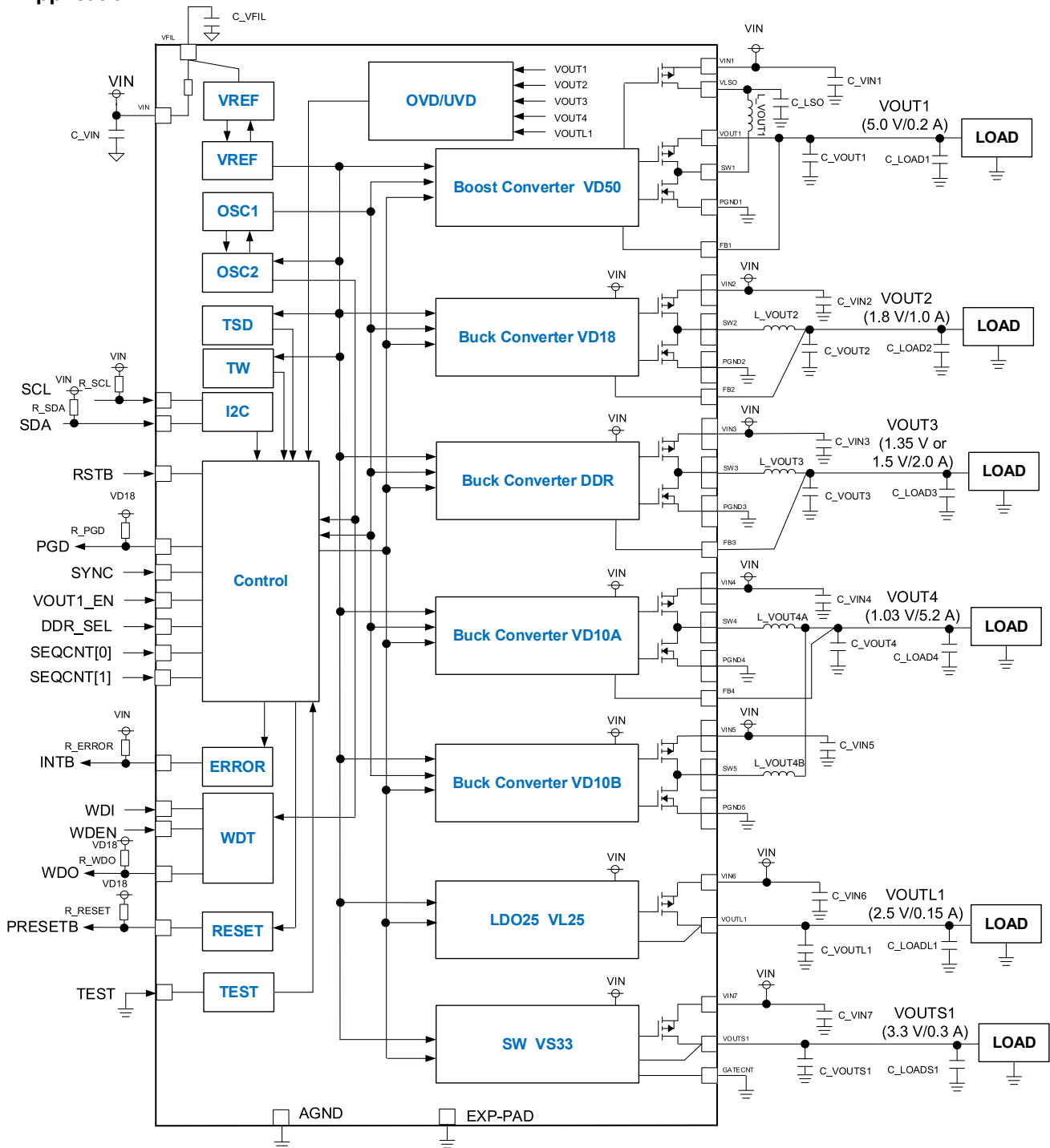
Figure 2. Application Circuit
