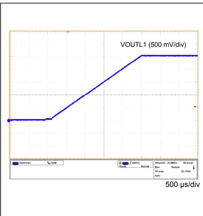
Figure 62. VOUTL1 Power ON Waveform
