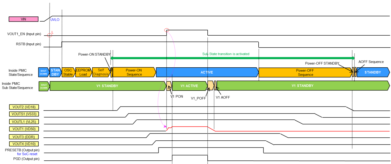
Figure 9. Whole Sequence1 (Mode B)
