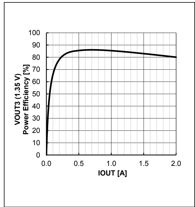
Figure 54. VOUT3 Power Efficiency vs IOU (VOUT3 = 1.35 V Setting)
