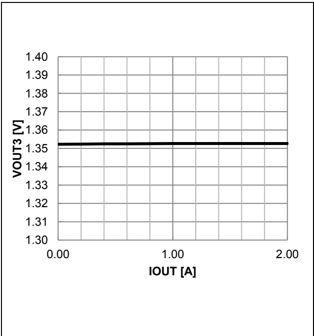
Figure 48. VOUT3 Output Voltage vs IOU (VOUT3 = 1.35 V Setting)
