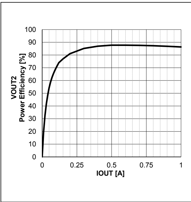
Figure 53. VOUT2 Power Efficiency vs IOU
