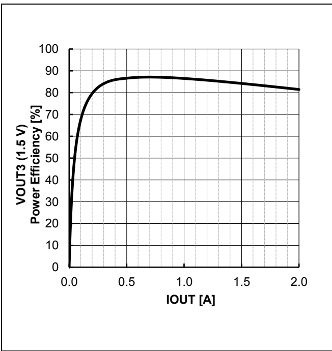
Figure 55. VOUT3 Power Efficiency vs IOU (VOUT3 = 1.5 V Setting)
