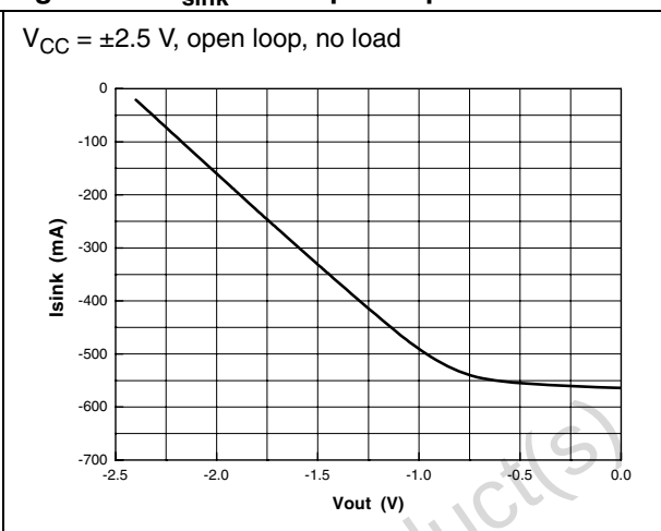
Figure 27. I_{\text{sink}} vs. output amplitude
