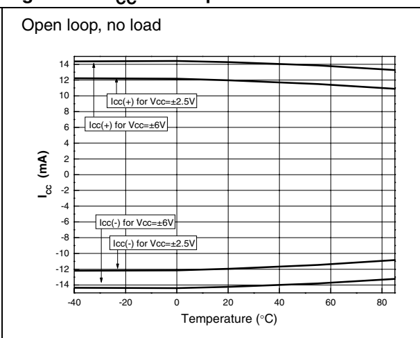
Figure 31. I_{\text{CC}} vs. temperature
