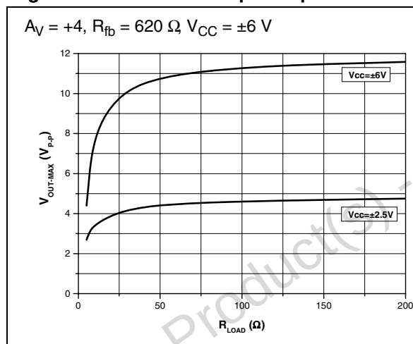
Figure 28. Maximum output amplitude vs. load
