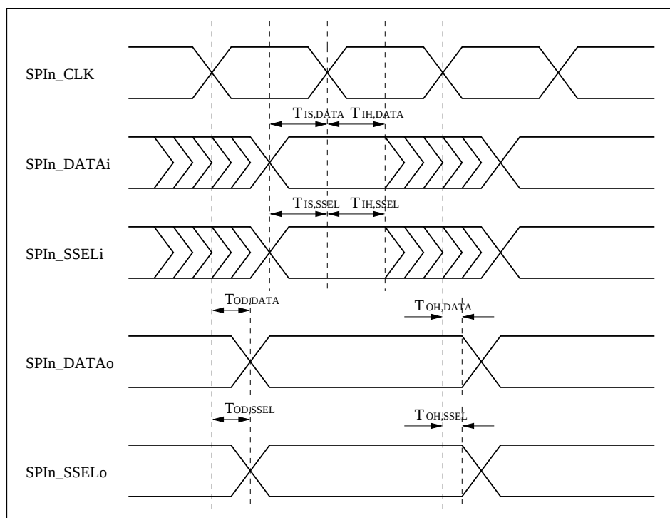
Figure 12. SPI Interface Timing
