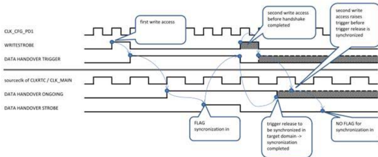
Figure 29. Handshake Synchronization
