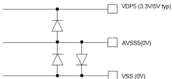
Figure 18. ESD Diodes between VDP5, AVSS5 and VSS
