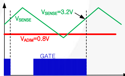
Figure 33. OCP Waveforms at V_{ADIM}=0.8 \text{ V}
