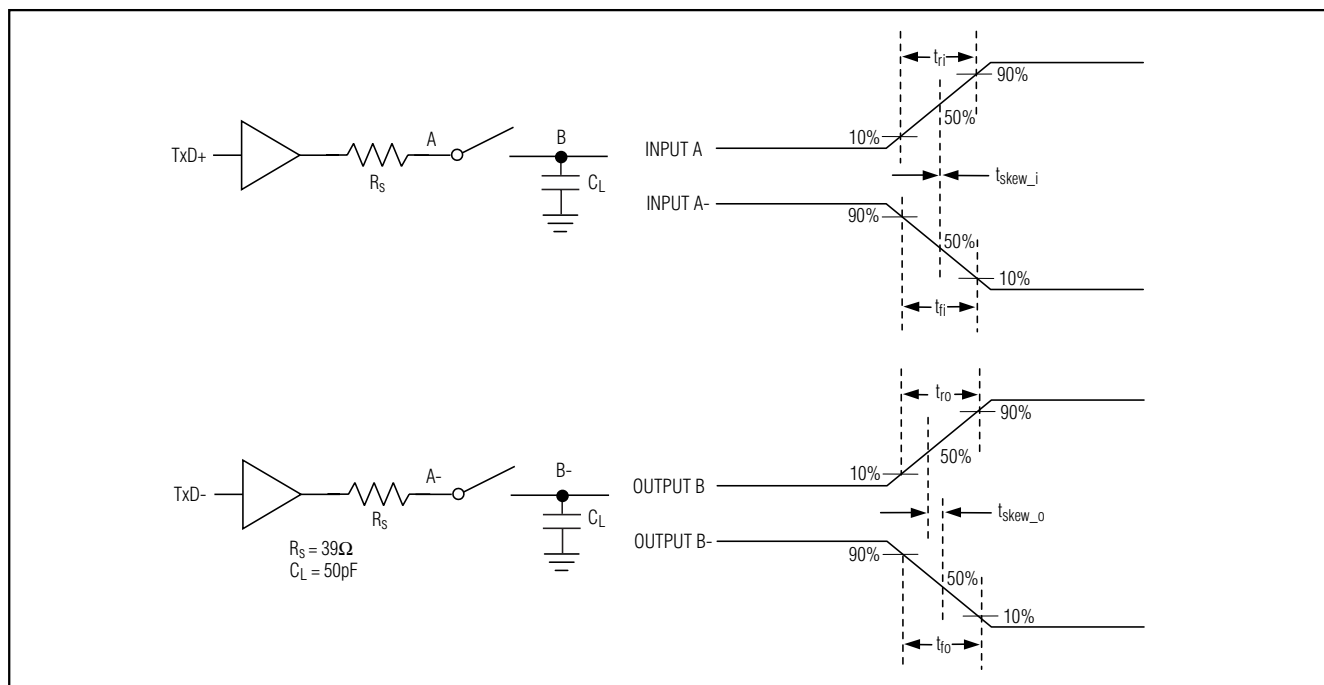
Figure 2. Input/Output Skew Timing Diagram
