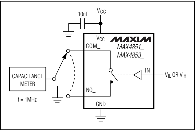
Figure 5. Channel Off-/On-Capacitance
