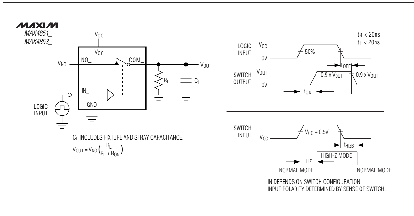
Figure 1. Switching Time
