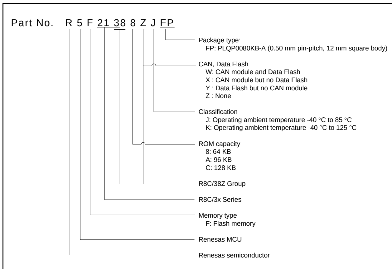
Figure 1.4 Part Number, Memory Size, and Package of R8C/38Z Group
