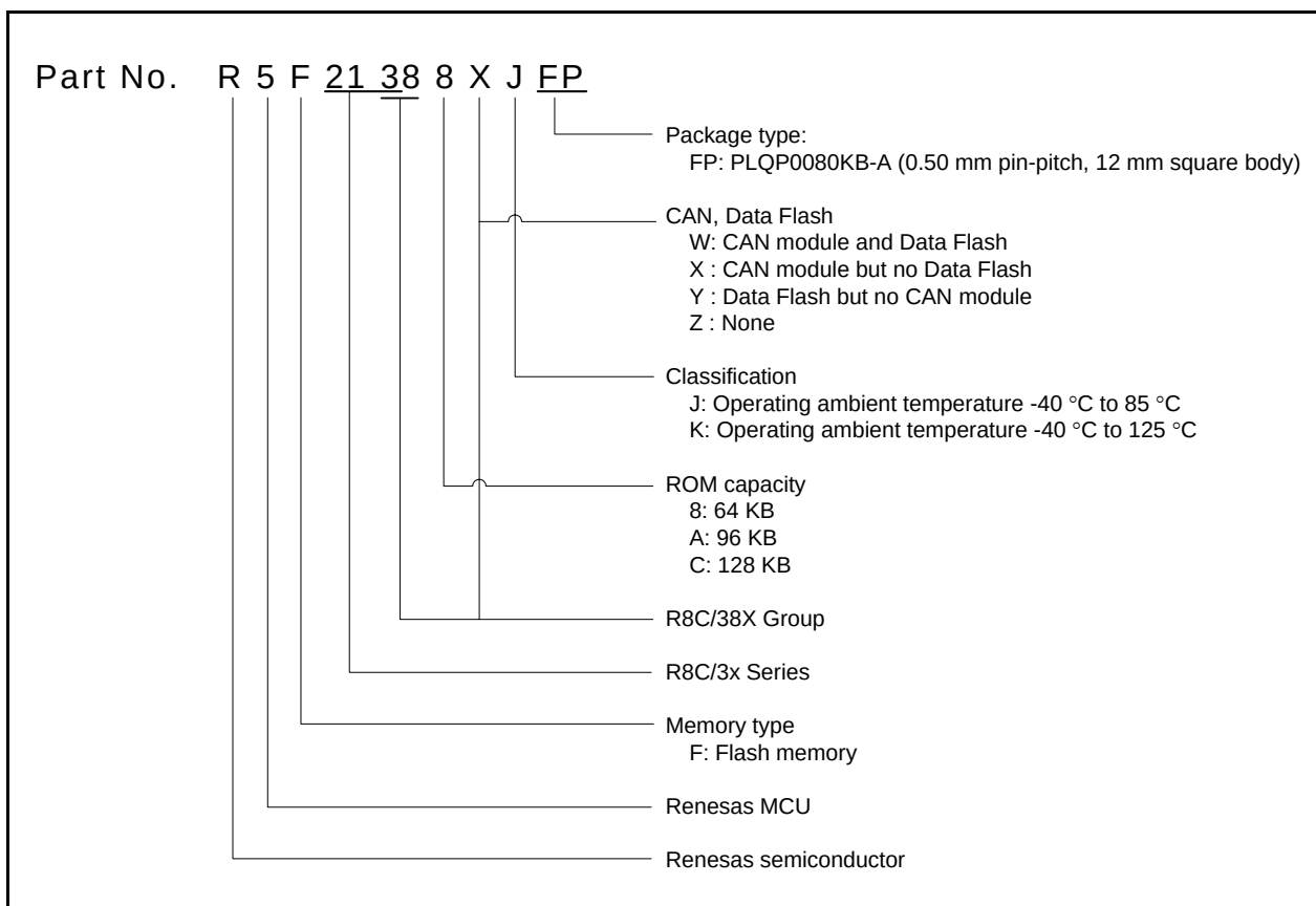
Figure 1.2 Part Number, Memory Size, and Package of R8C/38X Group
