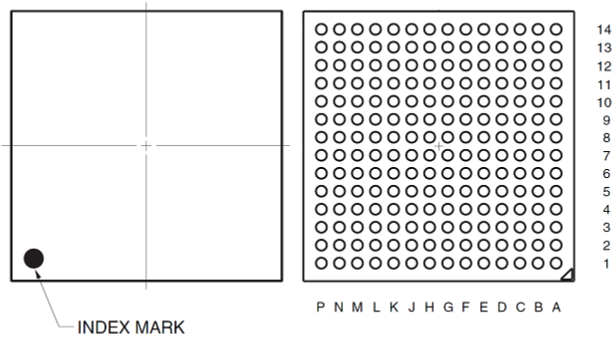
196-PIN PLASTIC BGA(15x15)
