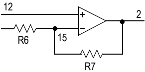
Figure 4. Adding Hysteresis
