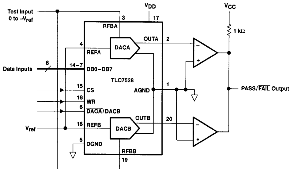
Figure 8. Digitally-Programmable Window Comparator (Upper- and Lower-Limit Tester)
