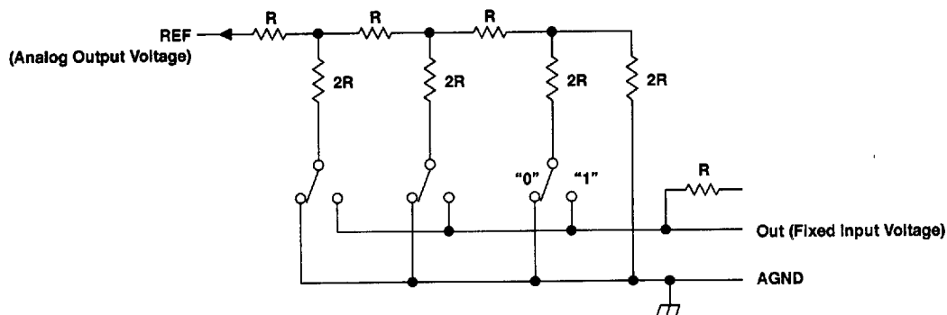
Figure 11. Voltage-Mode Operation
