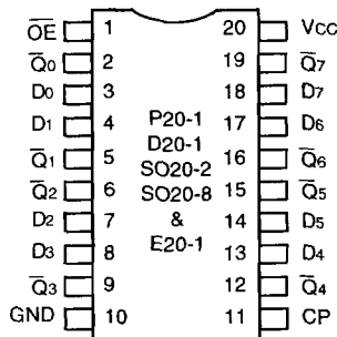
DIP/SSOP/SSOP/CSOP/CERPACK TOP VIEW
