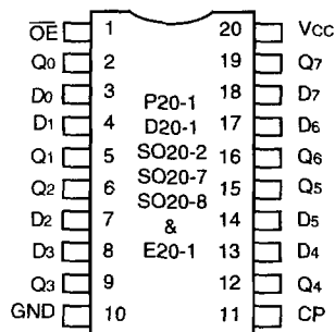
DIP/SSOP/SSOP/CSOP/CERPACK TOP VIEW
