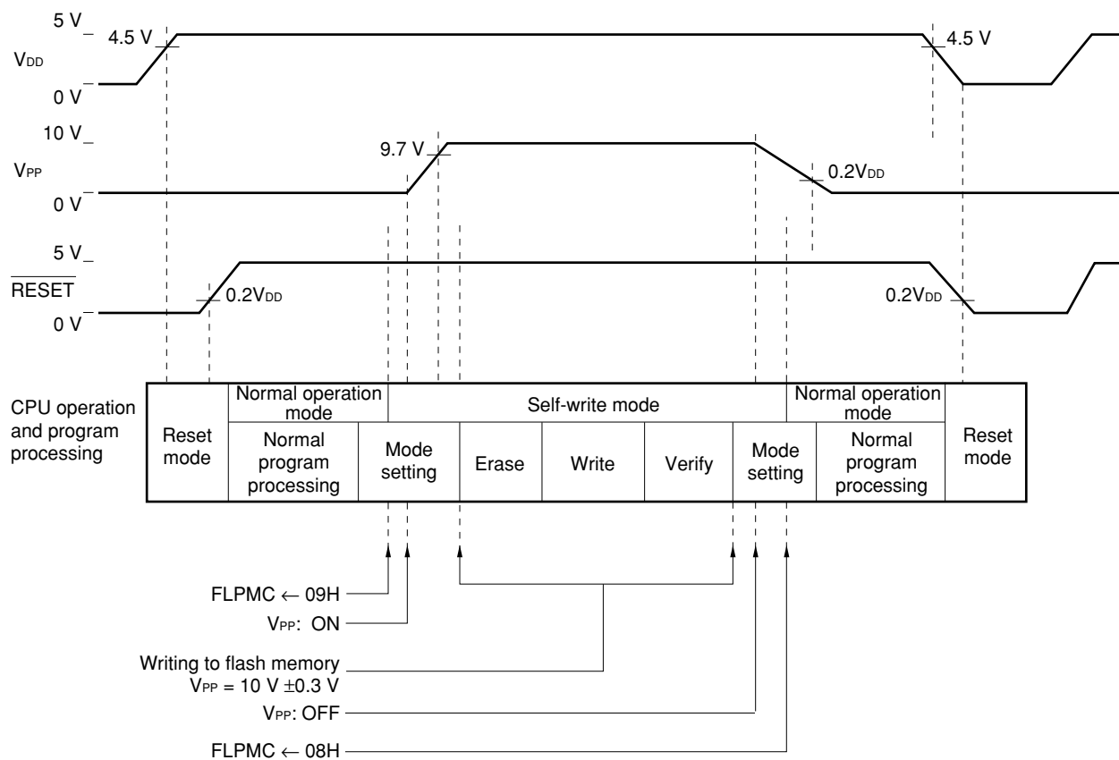
Figure 18-17. Self-Write Timing
