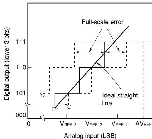
Figure 11-20. Full-Scale Error
