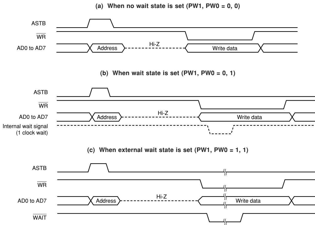
Figure 15-7. Write Timing of External Memory
