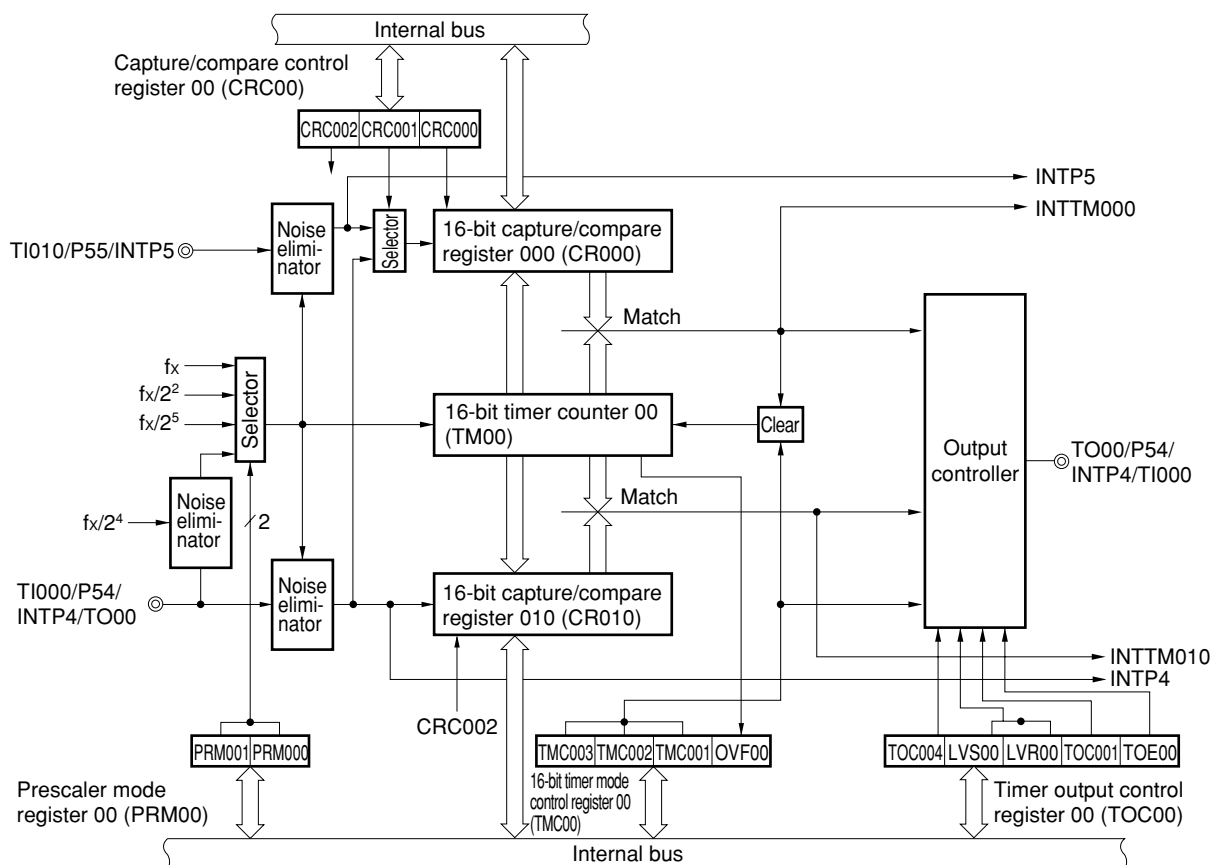
Figure 6-1. Block Diagram of 16-Bit Timer/Event Counter 00
