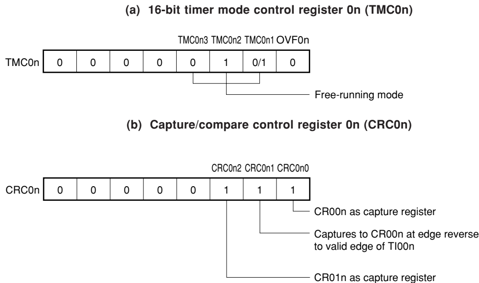
Figure 6-24. Control Register Settings for Pulse Width Measurement with Free-Running Counter and Two Capture Registers
