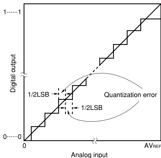
Figure 11-18. Quantization Error
