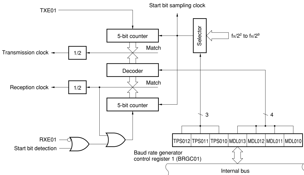
Figure 12-4. Block Diagram of UART01 Baud Rate Generator
