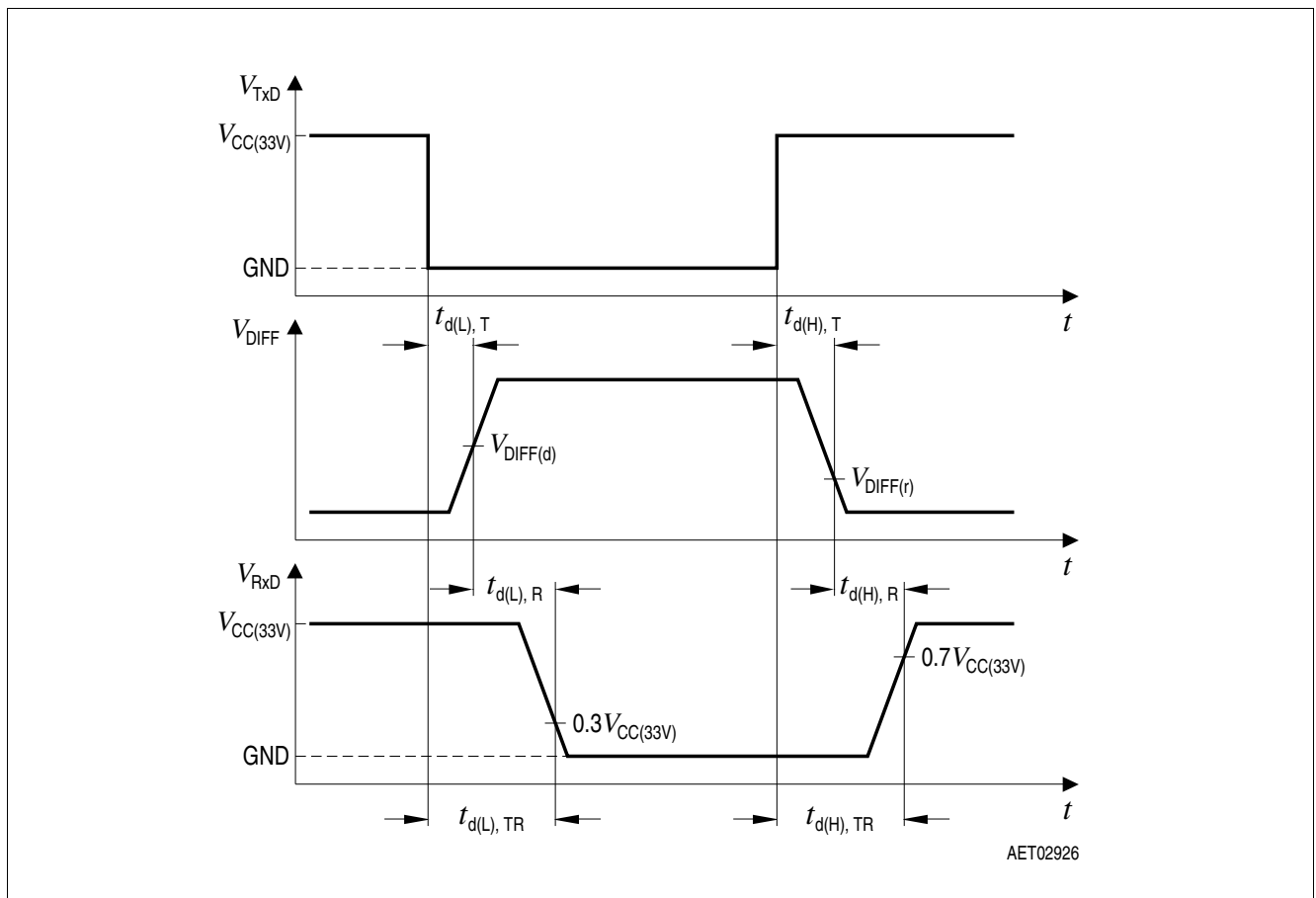
Figure 5 Timing Diagrams for Dynamic Characteristics
