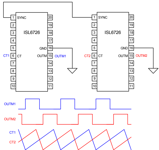
FIGURE 16. SYNCHRONIZING TWO UNITS
