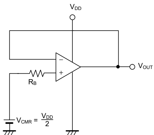
Figure 11 Test Circuit 9
