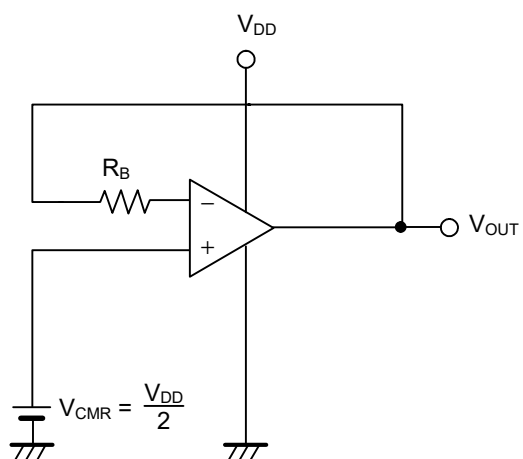
Figure 12 Test Circuit 10
