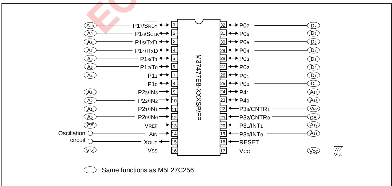
Fig. 32 Pin connection in EPROM mode
