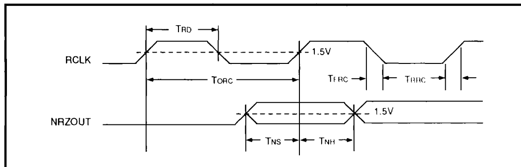
FIGURE 12: Read Mode Timing
