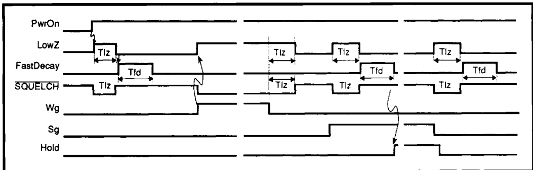
FIGURE 3: AGC Timing
