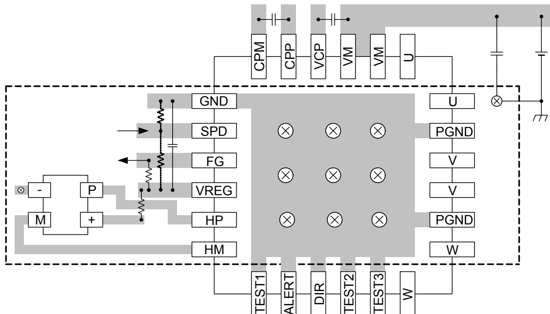
Figure 13.1 Reference Layout
