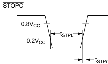
Figure 59 \overline{STOPC} Timing
