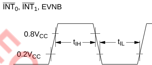
Figure 57 Interrupt Timing
