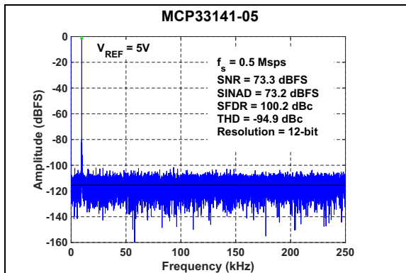
FIGURE 3-9: FFT for 10 kHz Input Signal: f_S = 500\text{ kps} , V_{IN} = -1\text{ dBFS} , V_{REF} = 5\text{V} .
