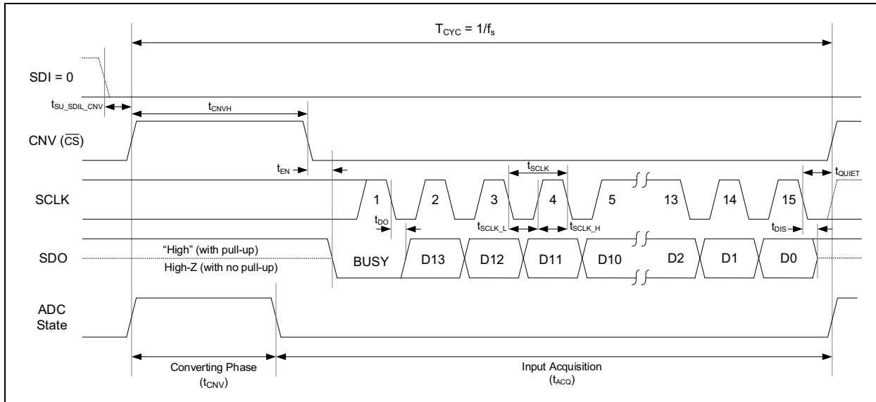
FIGURE 6-7: Timing Diagram for 3-Wire \overline{\text{CS}} Mode with BUSY Status Indicator Output Bit, Late \overline{\text{CNV}} .
