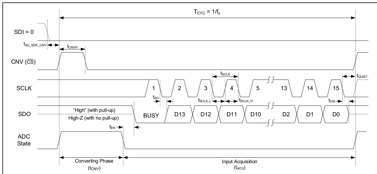
FIGURE 6-6: Timing Diagram for 3-Wire \overline{\text{CS}} Mode with \text{BUSY} Status Indicator Output Bit, Early \text{CNV} (Recommended).
