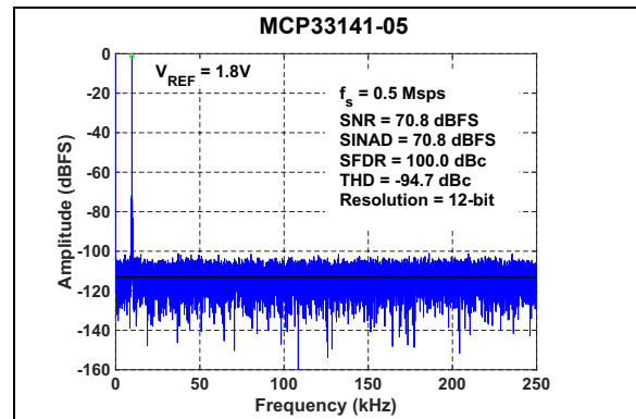
FIGURE 3-12: FFT for 10 kHz Input Signal: f_S = 500\text{ kps} , V_{IN} = -1\text{ dBFS} , V_{REF} = 1.8\text{V} .
