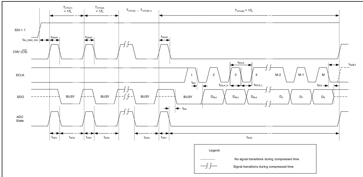
FIGURE 6-8: Interface Timing Diagram for Accumulator Operation in 3-Wire \overline{\text{CS}} Mode, with BUSY Status Indicator Output Bit.
