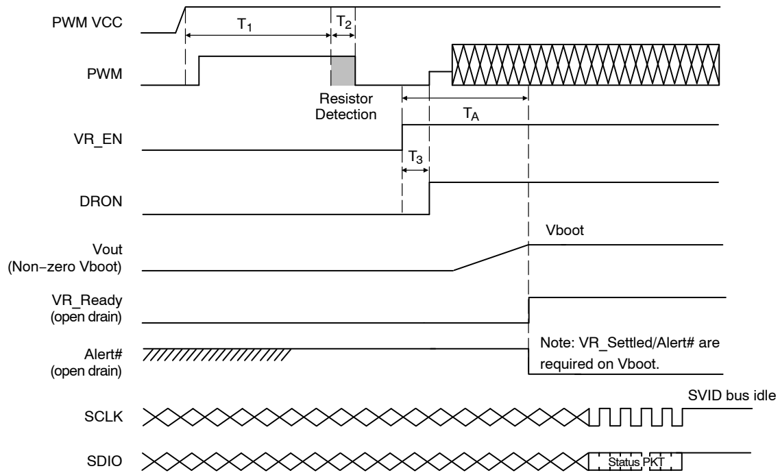
Figure 4. Start-Up Timing Diagram – VBOOT
