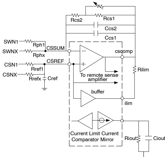
Figure 9. Total Current Sense Amplifier
