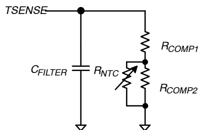
Figure 12. TSENSE Network
