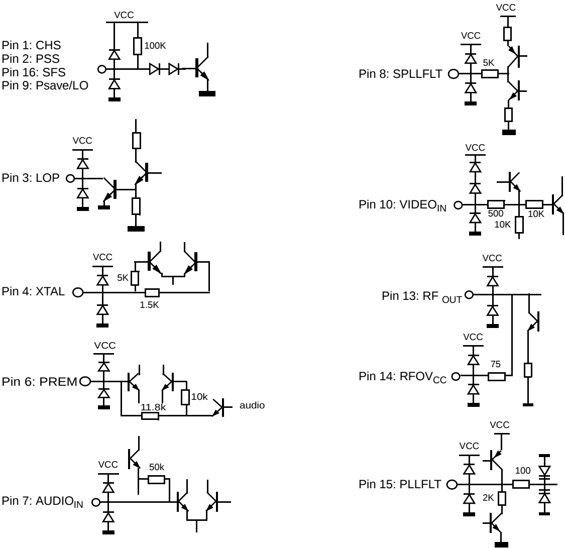
Figure 3. Pin Schematics
