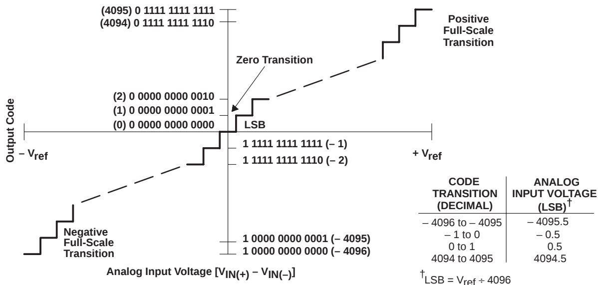
Figure 5. Transfer Characteristic
