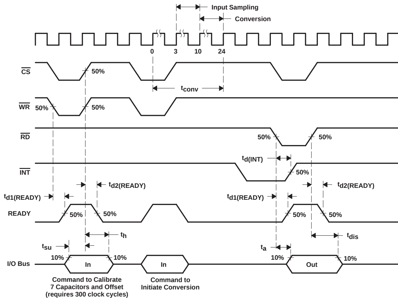
Figure 3. Timing Diagram
