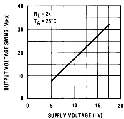
Voltage Swing
