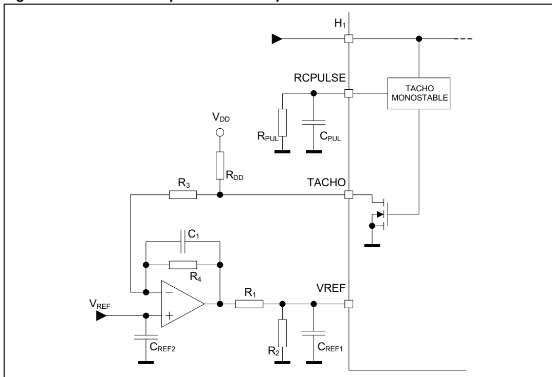
Figure 17. Tachometer speed control loop
