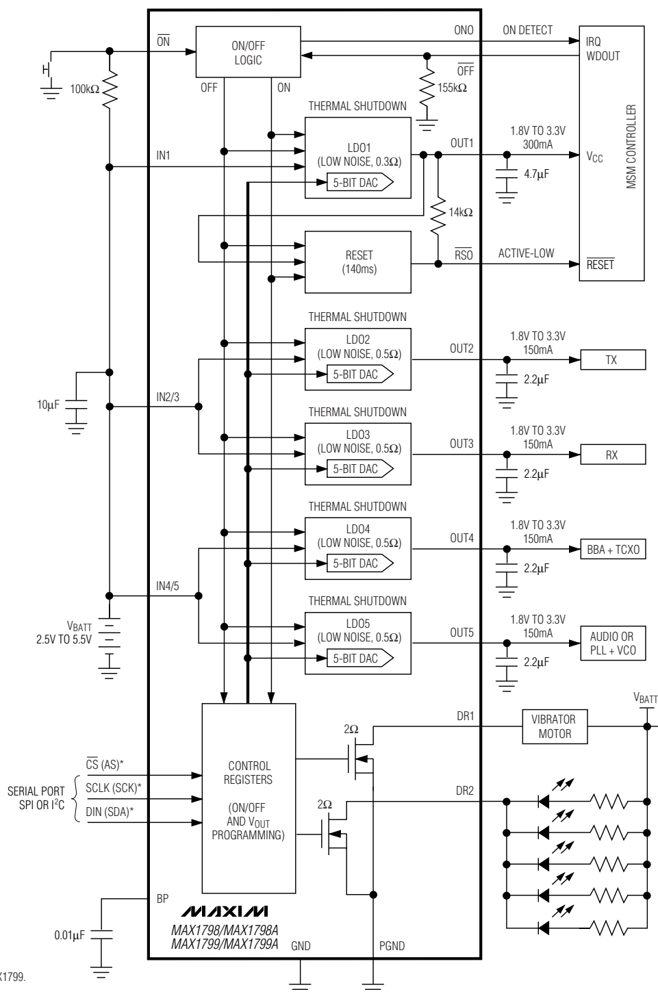
Figure 1. Typical Application Circuit/Functional Diagram
