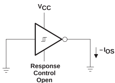
† Arrows indicate actual direction of current flow. Current into a terminal is a positive value.
