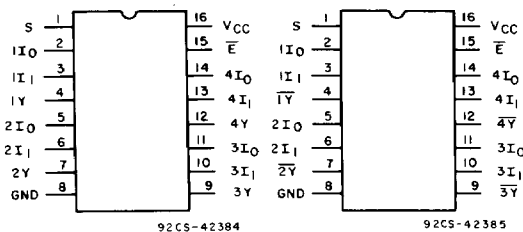
CD54/74AC/ACT157
