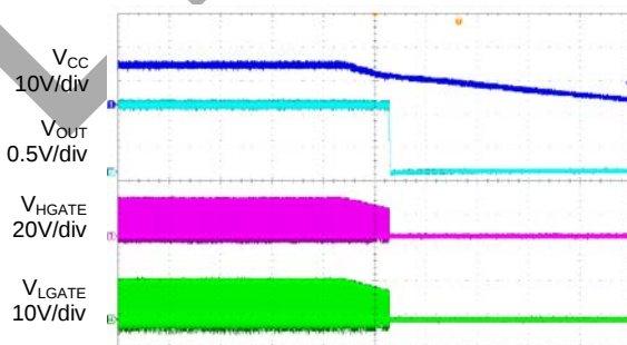
Power Off Waveform ( V_{IN}=12V , V_{OUT}=1.0V , I_{OUT}=60A )
