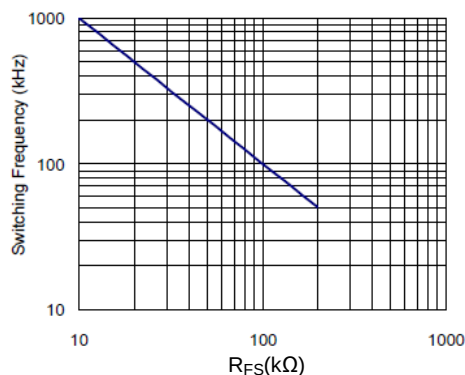
Figure 1. Switching Frequency vs. R_{FS}
