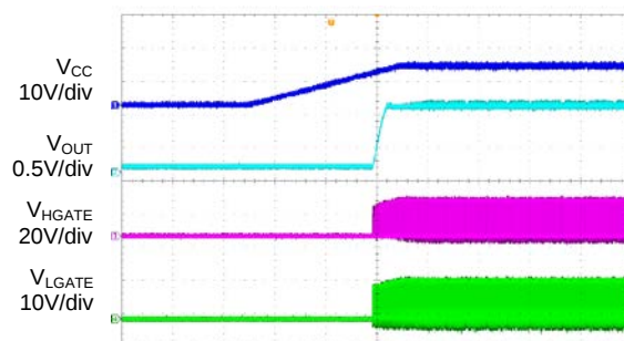
Power On Waveform ( V_{IN}=12V , V_{OUT}=1.0V , I_{OUT}=60A )
