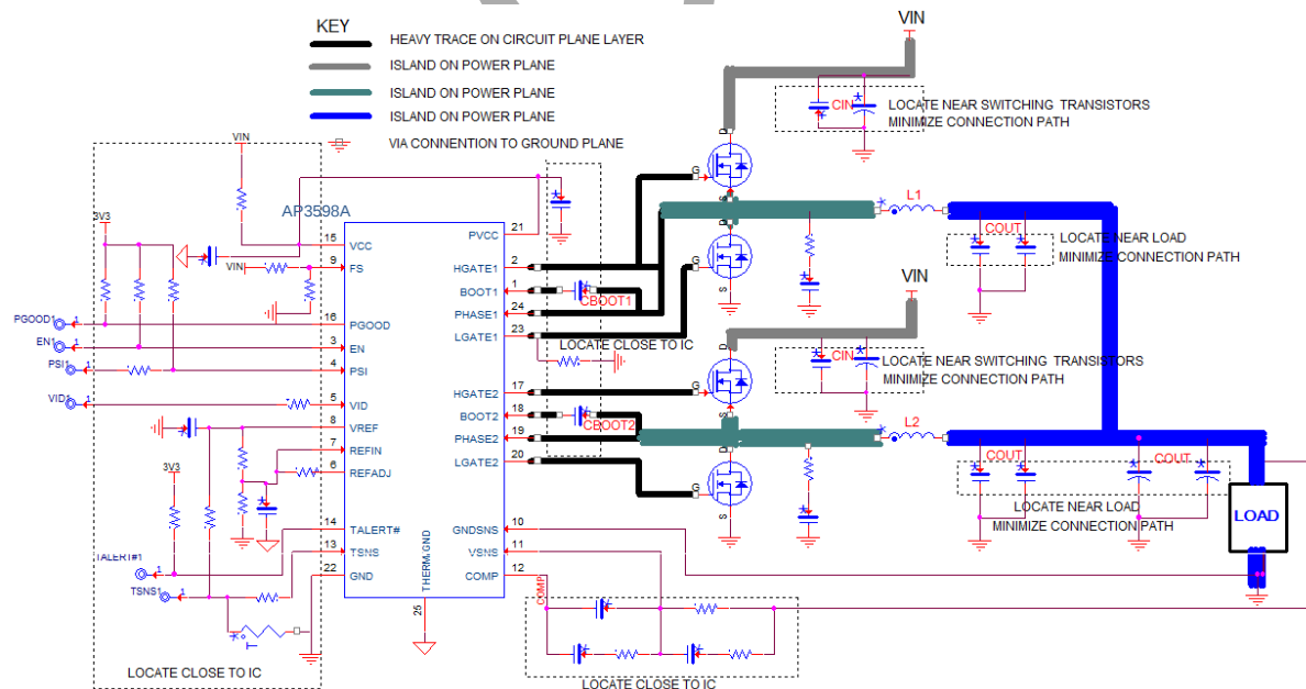
Figure 16. The Layout of AP3598A
