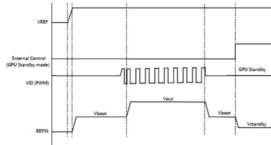
Figure 8. Time Diagram
