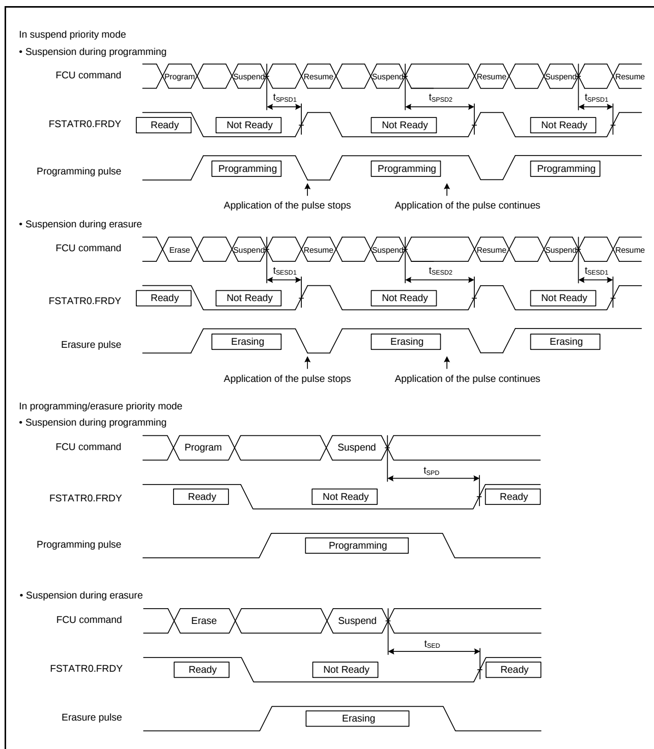
Figure 5.57 Flash Memory Program/Erase Suspend Timing
