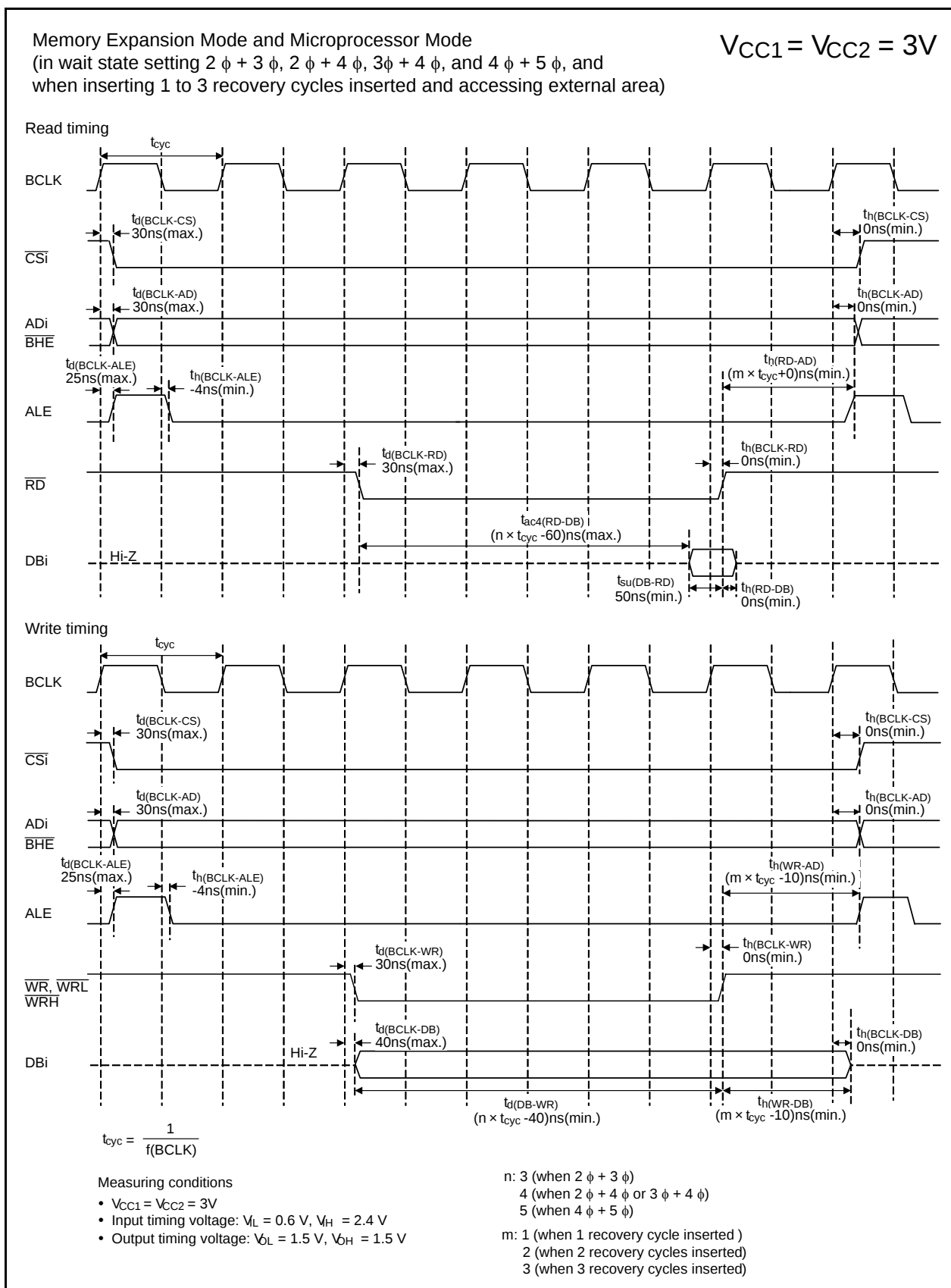
Figure 5.35 Timing Diagram
