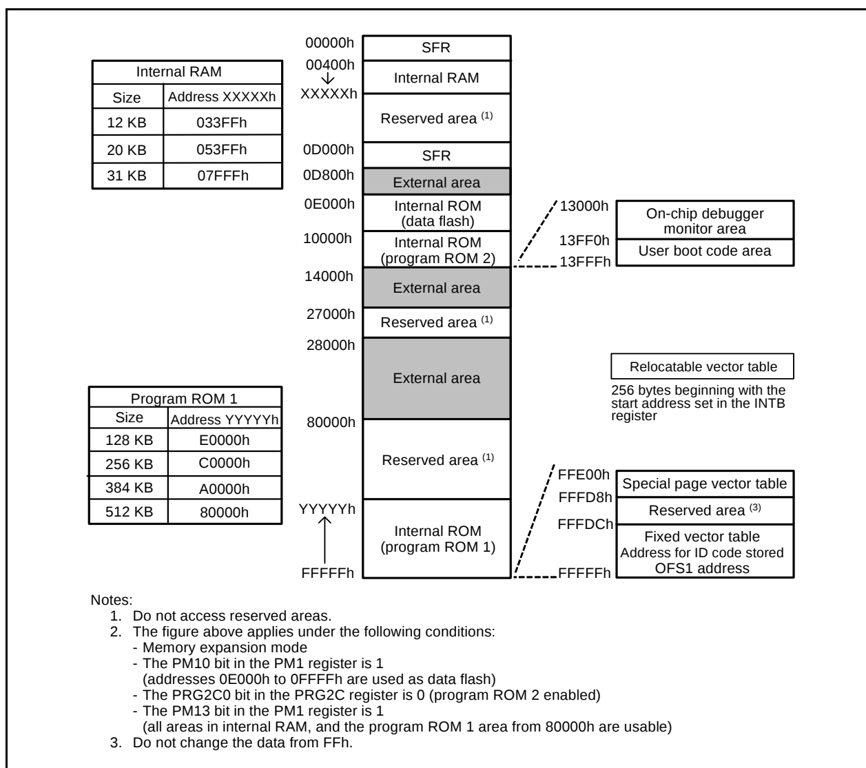
Figure 3.2 Memory Map
