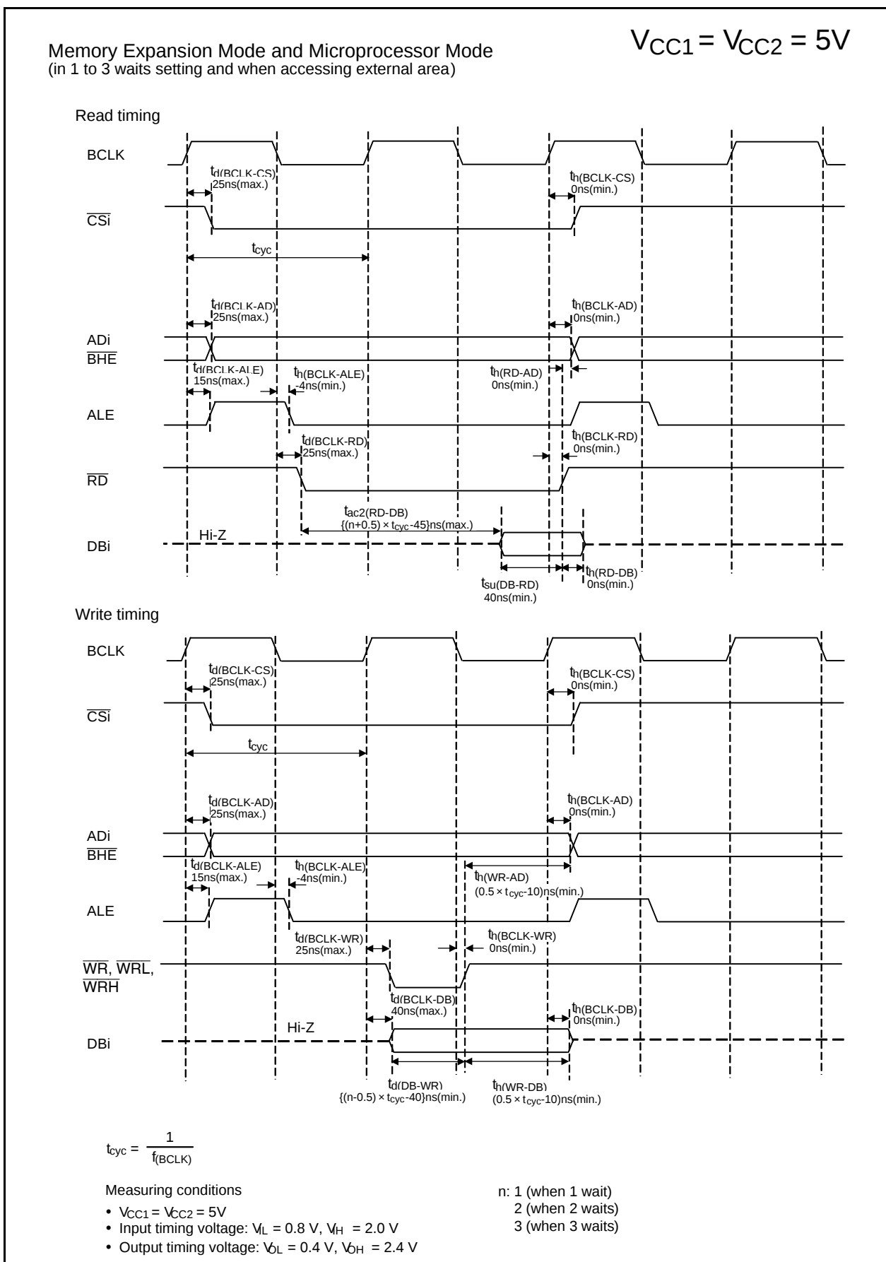
Figure 5.17 Timing Diagram
