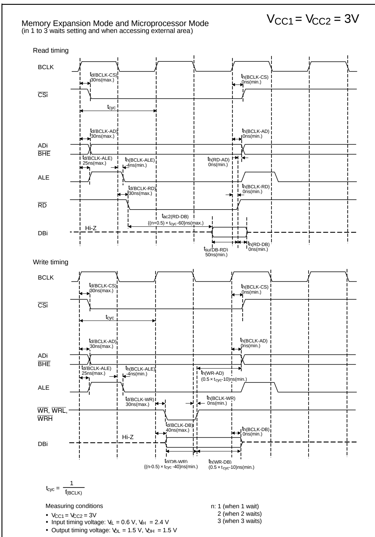
Figure 5.32 Timing Diagram
