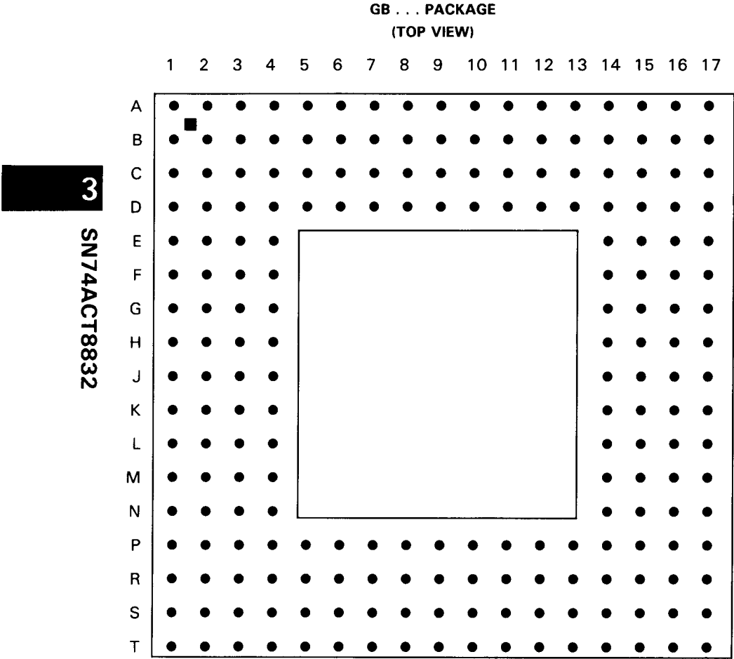
Figure 2. SN74ACT8832 . . . GB Package
