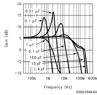
Closed Loop Frequency Response vs Capacitive Load ( A_V = +2 , V_S = \pm 5\text{V} )
