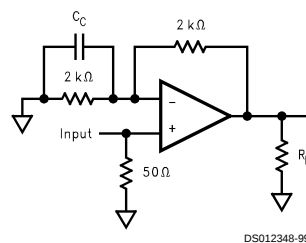
(b) A_V = +2
