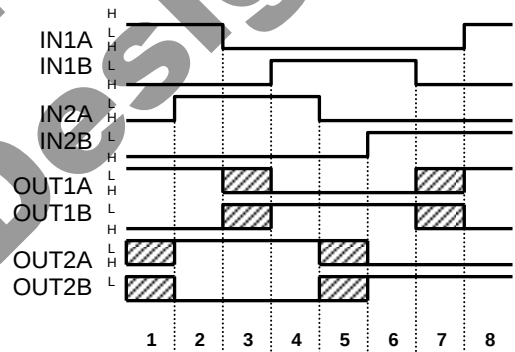
Figure 6. 1-2 Phases Timing Sequence with IN/IN Input
