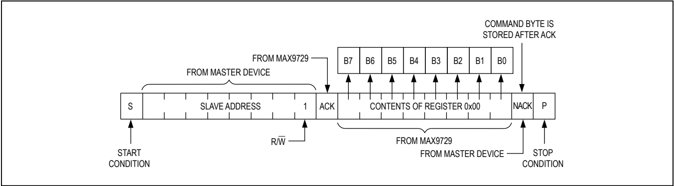
Figure 7a. Read Data Format for Reading Register 0x00 Only
