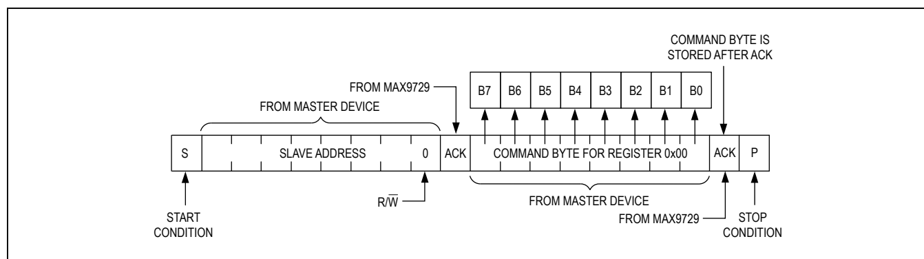
Figure 6a. Write Data Format for Writing to Register 0x00 Only
