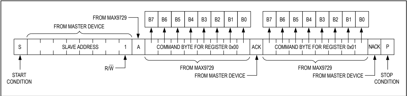
Figure 7b. Read Data Format for Reading Registers 0x00 and 0x01
