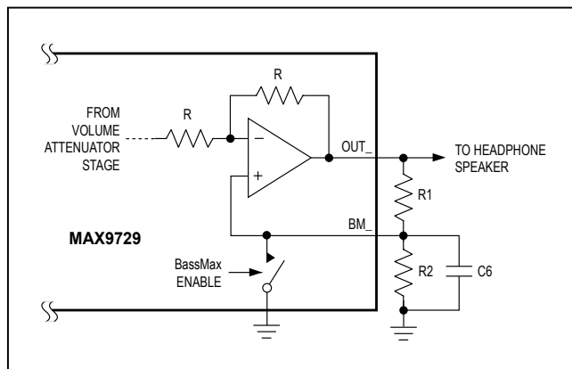
Figure 2. BassMax External Connections
