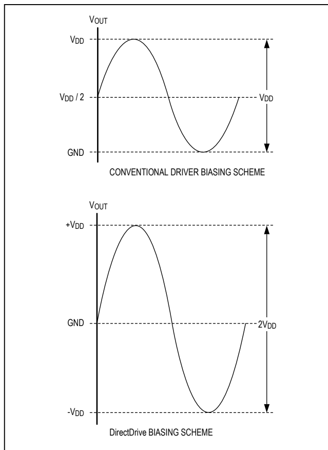
Figure 1. Traditional Amplifier Output vs. MAX9729 DirectDrive Output
