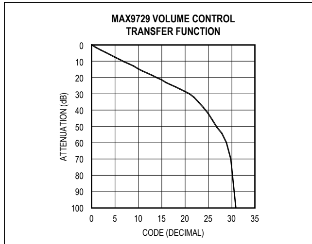
Figure 8. MAX9729 Volume Control Transfer Function
