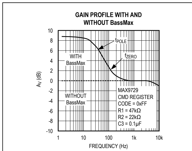
Figure 9. BassMax Gain Profile Example
