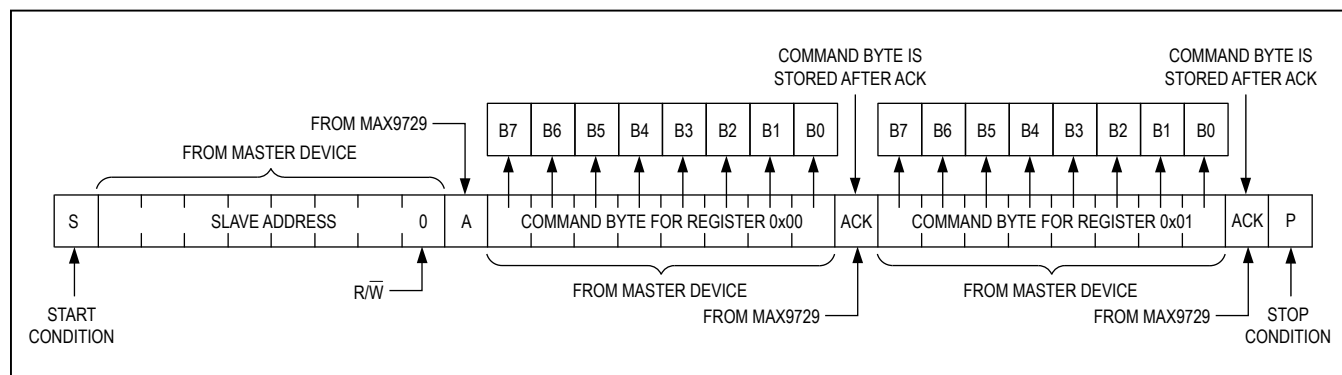
Figure 6b. Write Data Format for Writing to Registers 0x00 and 0x01
