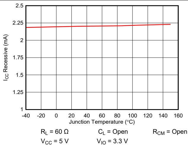
Figure 7-2. I_{CC} Recessive vs Temperature
