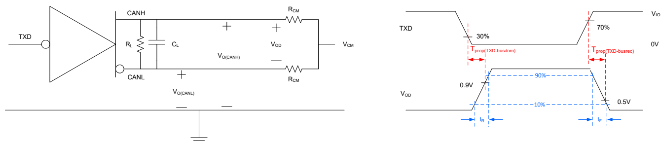
Figure 8-4. Driver Test Circuit and Measurement
