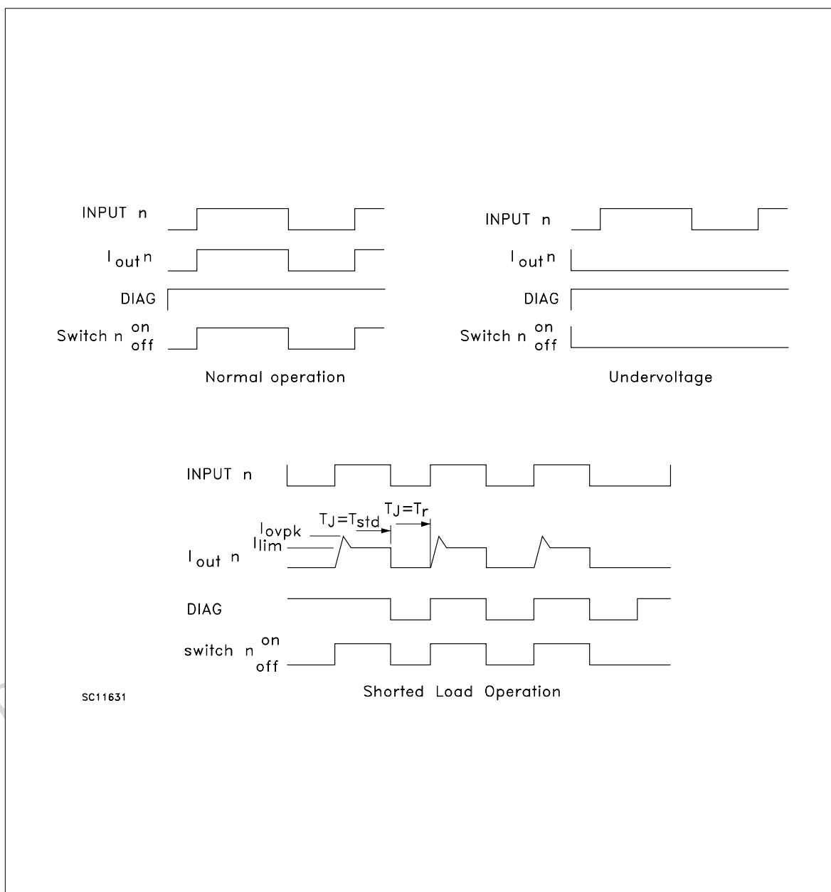
Figure 3: Switching Waveforms
