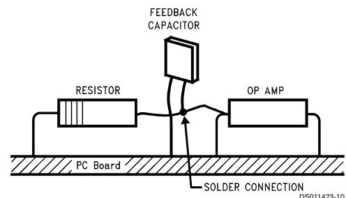
FIGURE 6. Air Wiring
