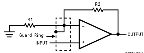
Non-Inverting Amplifier
