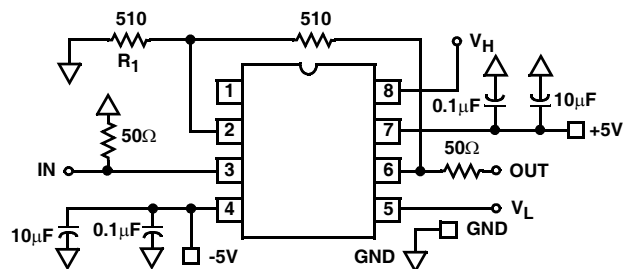
FIGURE 2C. SCHEMATIC
