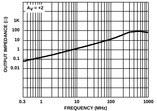
FIGURE 20. OUTPUT IMPEDANCE
