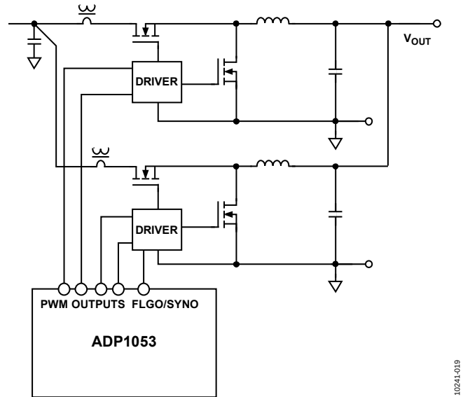
Figure 20. Phase Shedding in Dual-Phase Buck Controller
