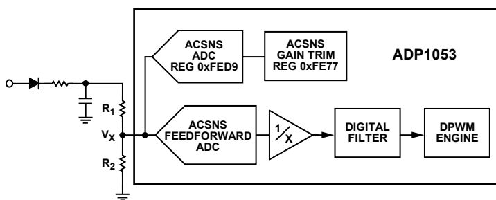
Figure 19. Feedforward Configuration
