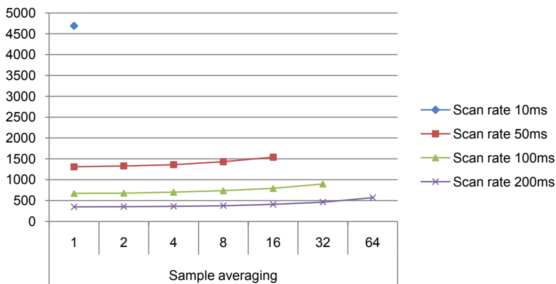
Figure 37-12. Power Consumption [ \mu A] 100 sensors, noise countermeasures Enabled, f=48\text{MHz} , V_{cc}=3.3\text{V}
