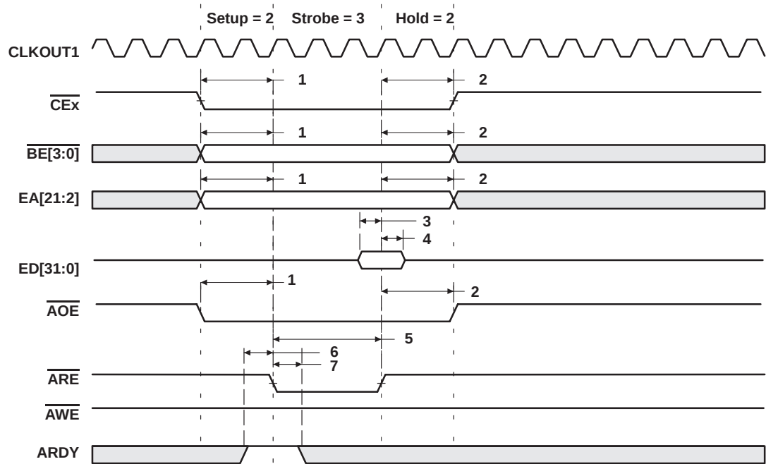
Figure 16. Asynchronous Memory Read Timing (ARDY Not Used)
