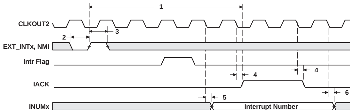
Figure 30. Interrupt Timing
