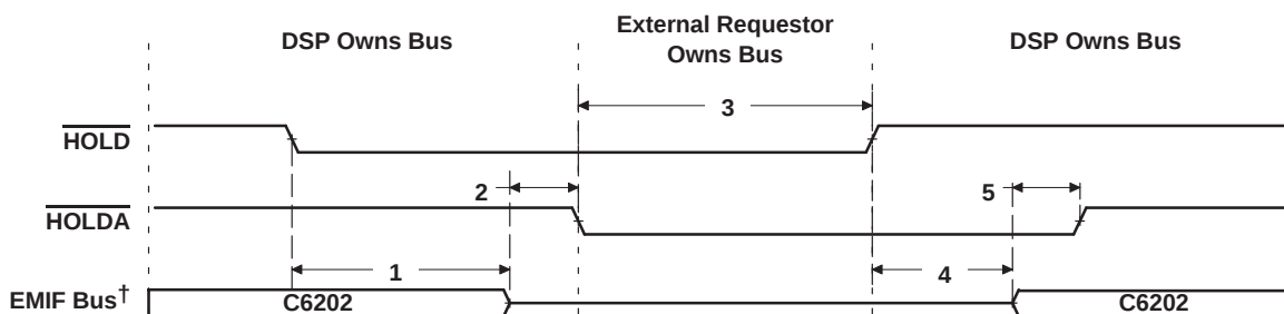
Figure 28. HOLD/HOLDA Timing
