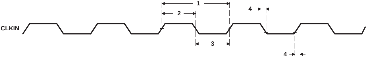
Figure 12. CLKIN Timings
