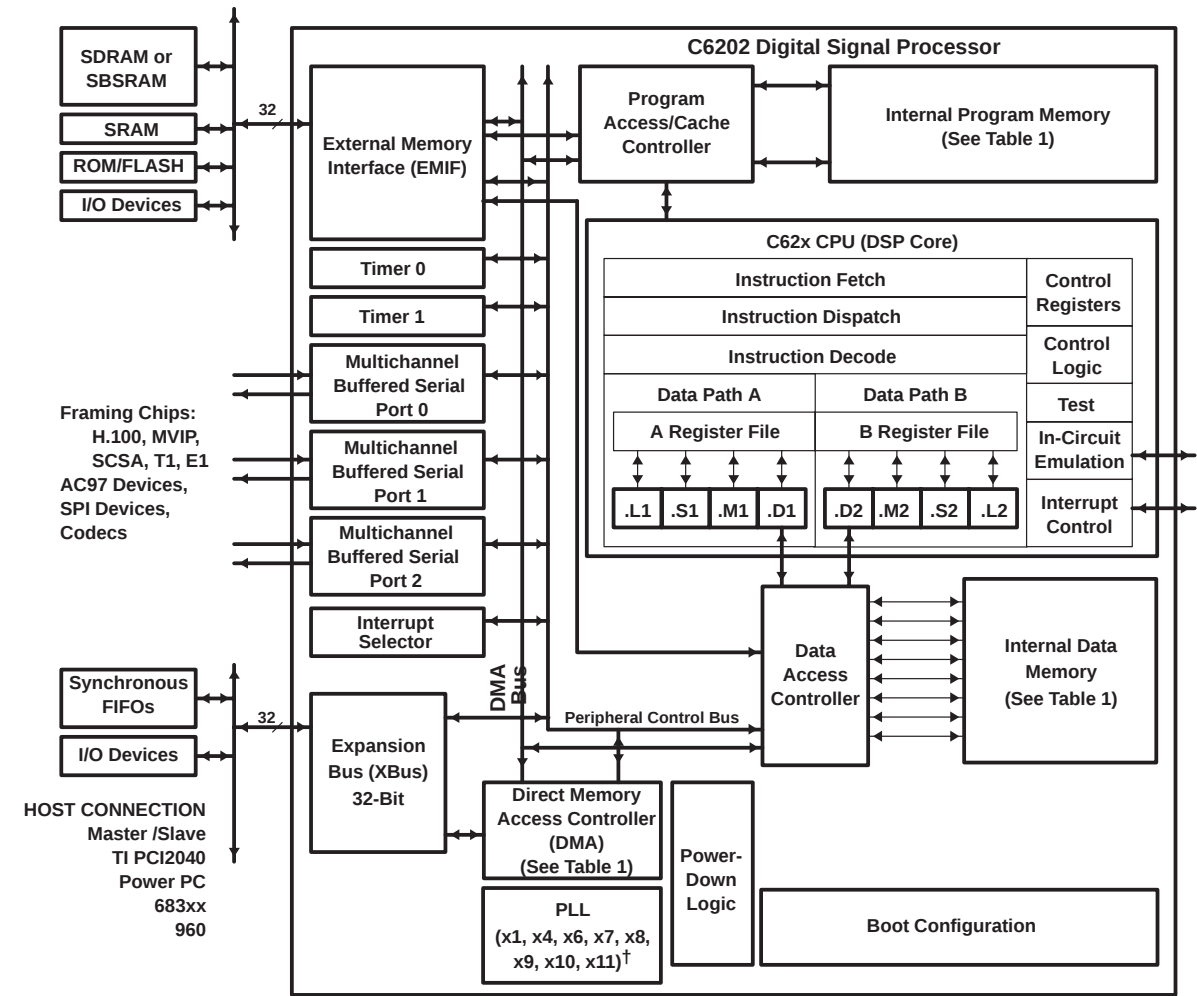
functional and CPU (DSP core) block diagram
