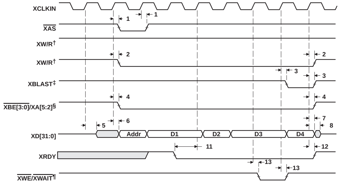
Figure 40. C62x™ as Bus Master—Read
