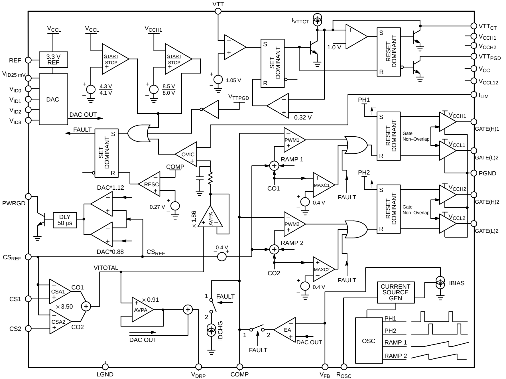
Figure 2. Block Diagram
