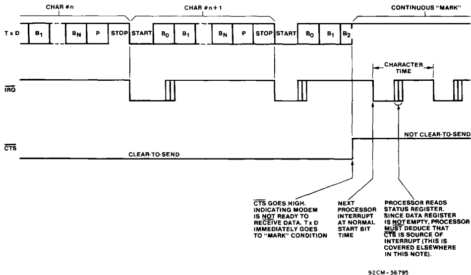
Fig. 10 - Effect of CTS on CDP65C51 transmitter
