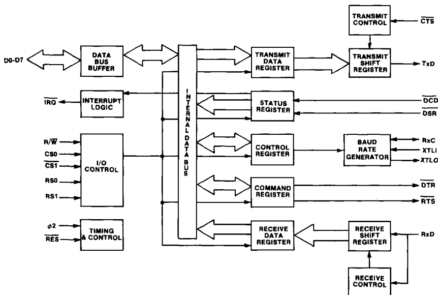
Fig. 2 - Internal organization.
