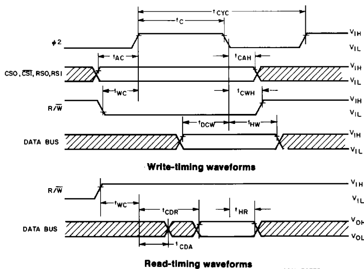
Fig. 22 - Timing waveforms.
