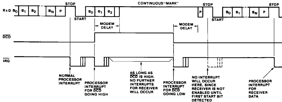
Fig. 16 - Effect of DCD on receiver.
