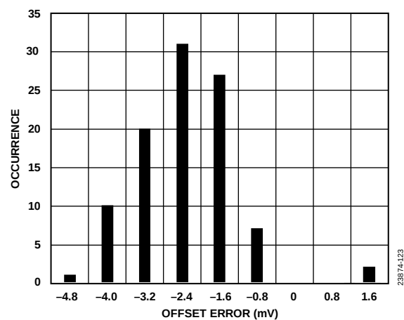
Figure 15. Offset Error Distribution Histogram
