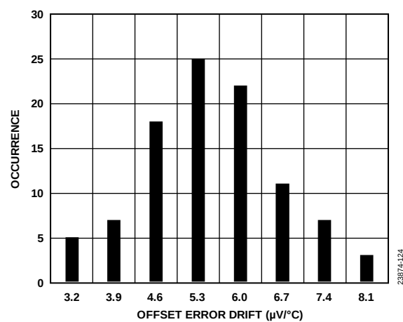
Figure 16. Offset Error Drift Distribution Histogram
