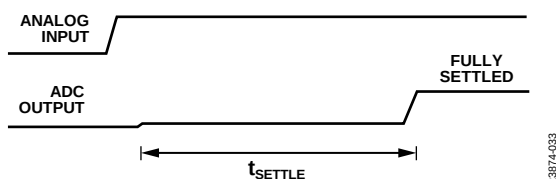
Figure 33. Step Input with Single Cycle Settling
