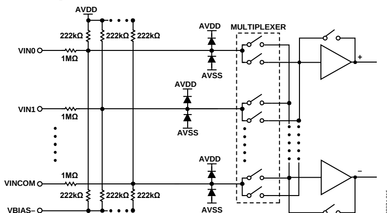
Figure 25. Simplified Voltage Input Circuit
