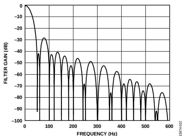
Figure 34. 27.27 SPS ODR, 36.67 ms Settling Time
