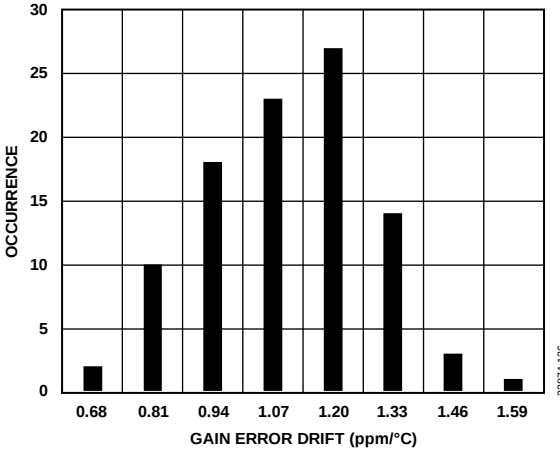
Figure 18. Gain Error Drift Distribution Histogram
