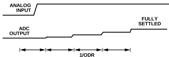
Figure 32. Step Input Without Single-Cycle Settling
