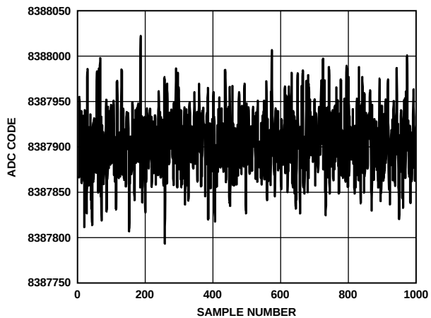
Figure 7. Noise (Output Data Rate = 125 kSPS)
