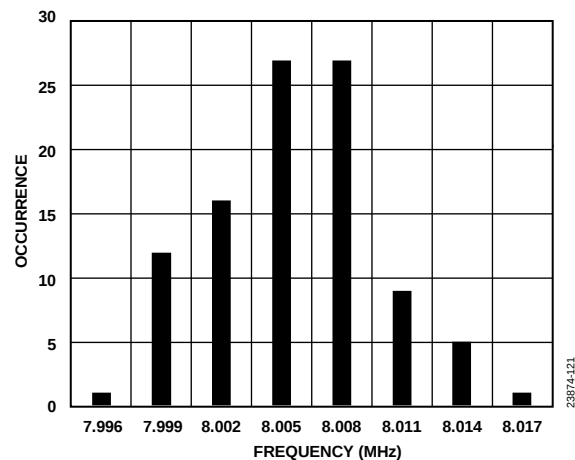
Figure 14. Internal Oscillator Frequency and Accuracy Distribution Histogram
