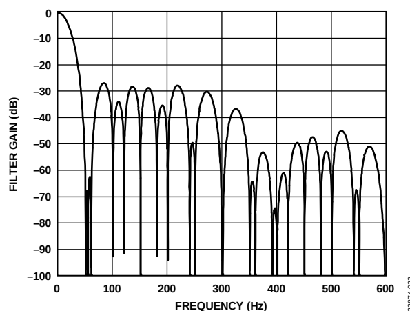
Figure 35. 25 SPS ODR, 40 ms Settling Time
