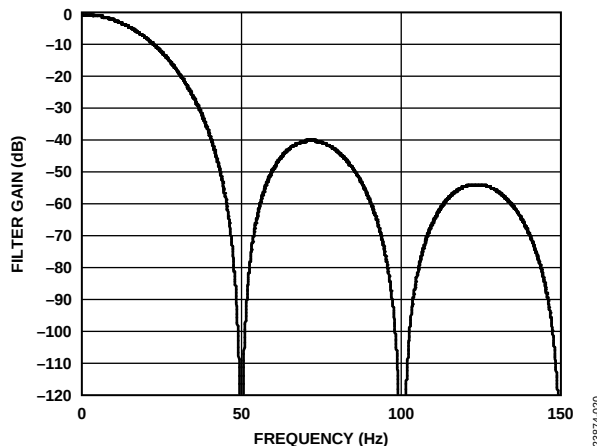
Figure 31. Sinc3 Filter Response
