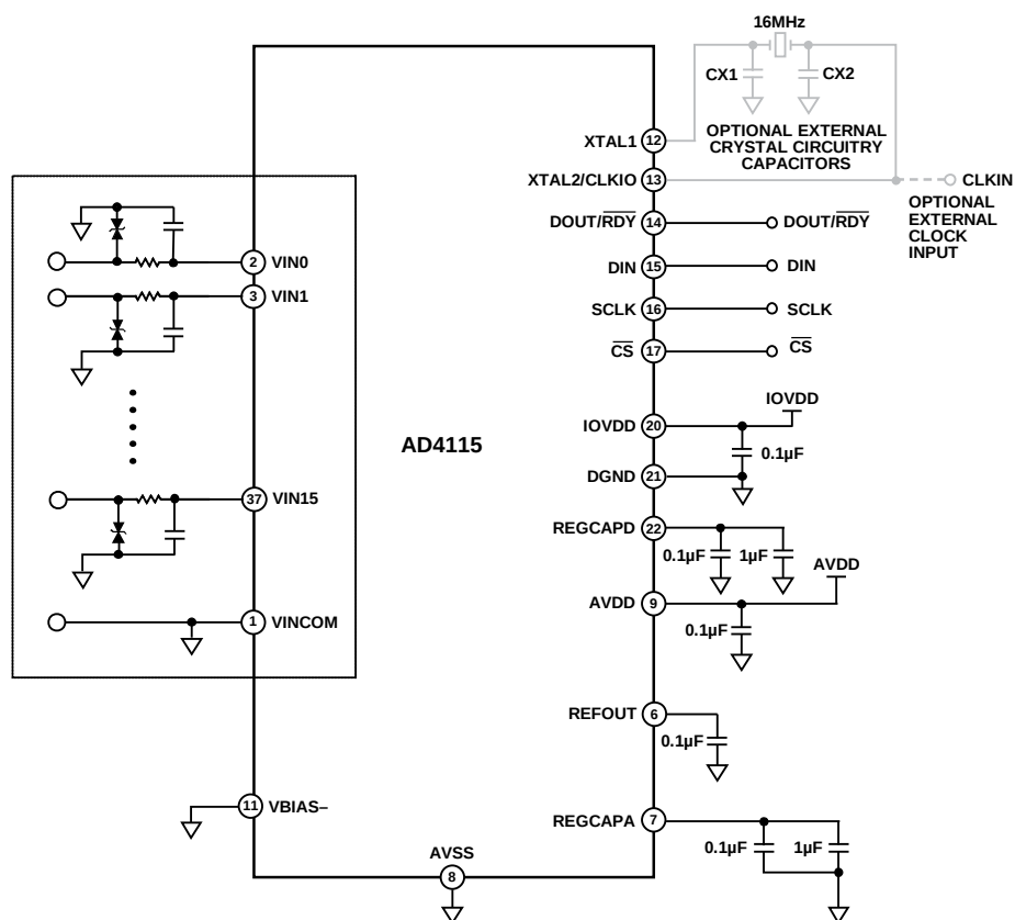
Figure 19. Typical Connection Diagram
