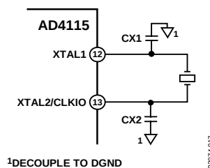
Figure 28. External Crystal Connections
