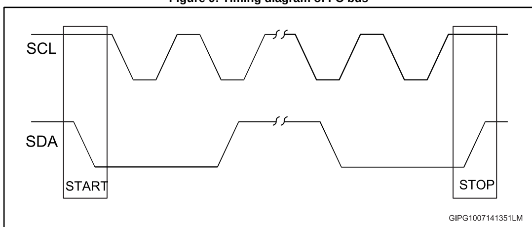
Figure 9: Timing diagram of I 2 C bus
