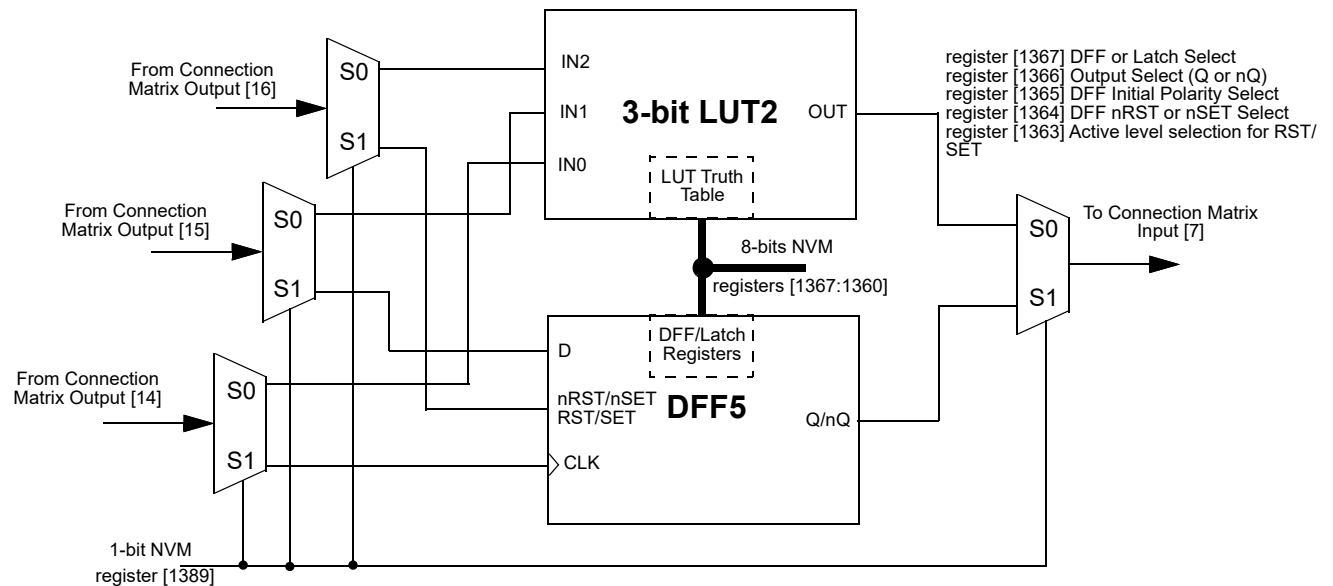
Figure 27: 3-bit LUT2 or DFF5
