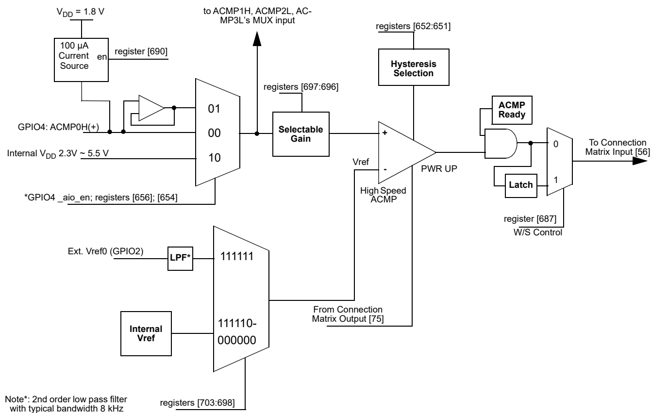
Figure 66: ACMP0H Block Diagram
