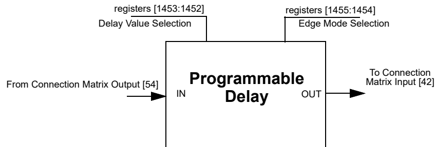
Figure 76: Programmable Delay
