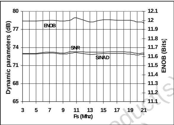
Fig. 14: Distortion vs. Fs at Fin=5MHz, using TS4041 lcca optimised; VREFP=1.225V; VREFM=GND; INCM=0.65V
