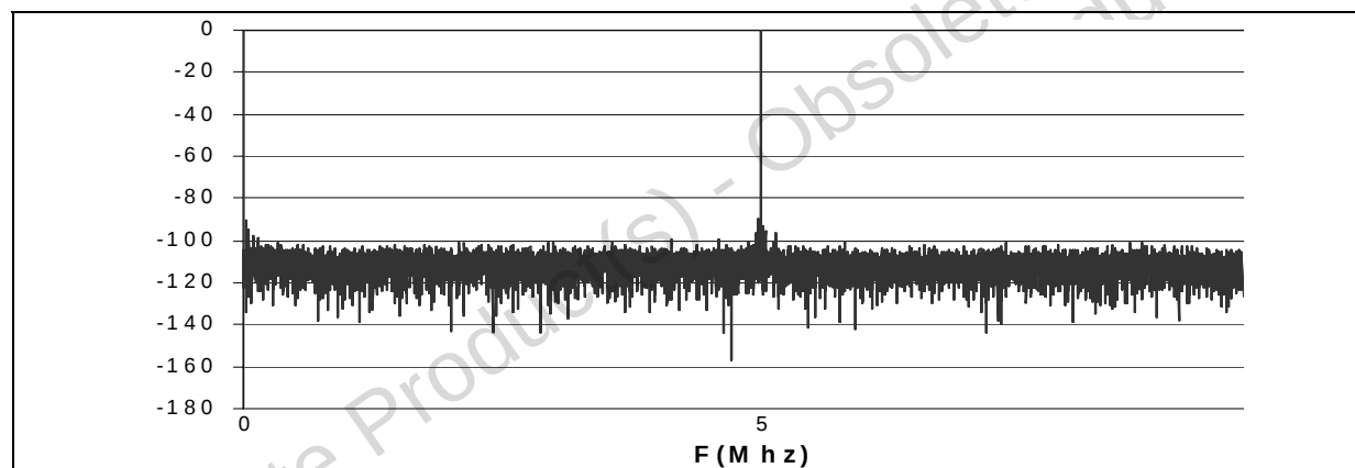
Fig. 9: Single-tone 16K FFT at F_s=20\text{MSPS} , External References TS4041
