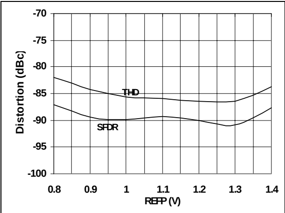
Fig. 11: Distortion vs. VREFP Fin=5MHz;Fs=20Mhz;lcca=26mA;INCM=0.46V
