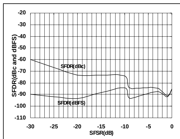
Fig. 8: Single-tone 16K FFT at F_s=20\text{ Msp} s, Internal references
