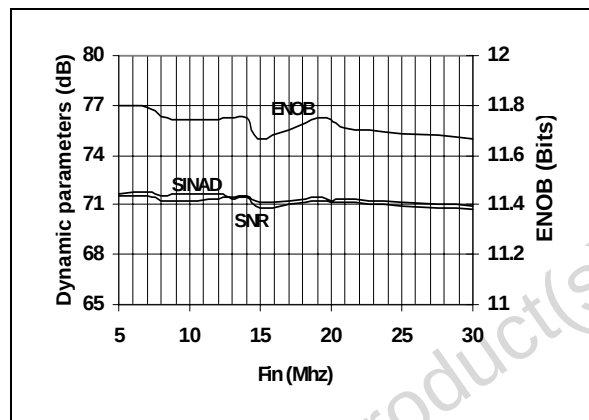
Fig. 5: Distortion vs. Fin, External References
