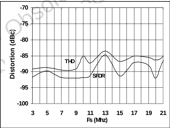
Fig. 14: Distortion vs. Fs at Fin=5MHz, using TS4041 lcca optimised; VREFP=1.225V; VREFM=GND; INCM=0.65V
