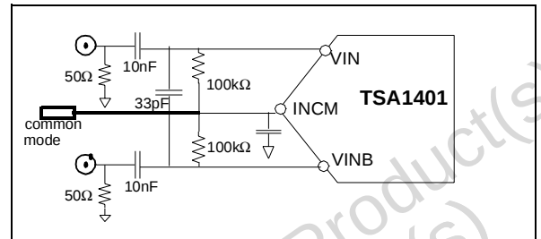
Fig. 17: AC-coupled differential input
