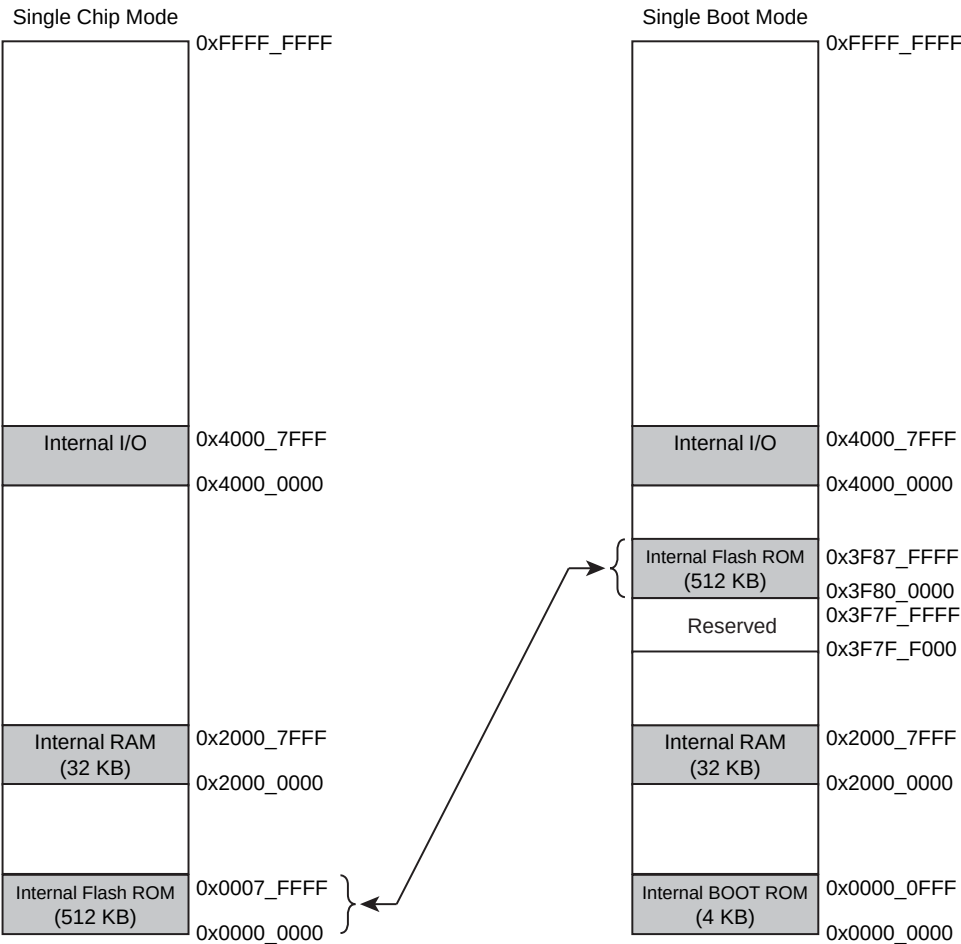
Figure 17-3 Memory Maps for TMPM330FDFG
