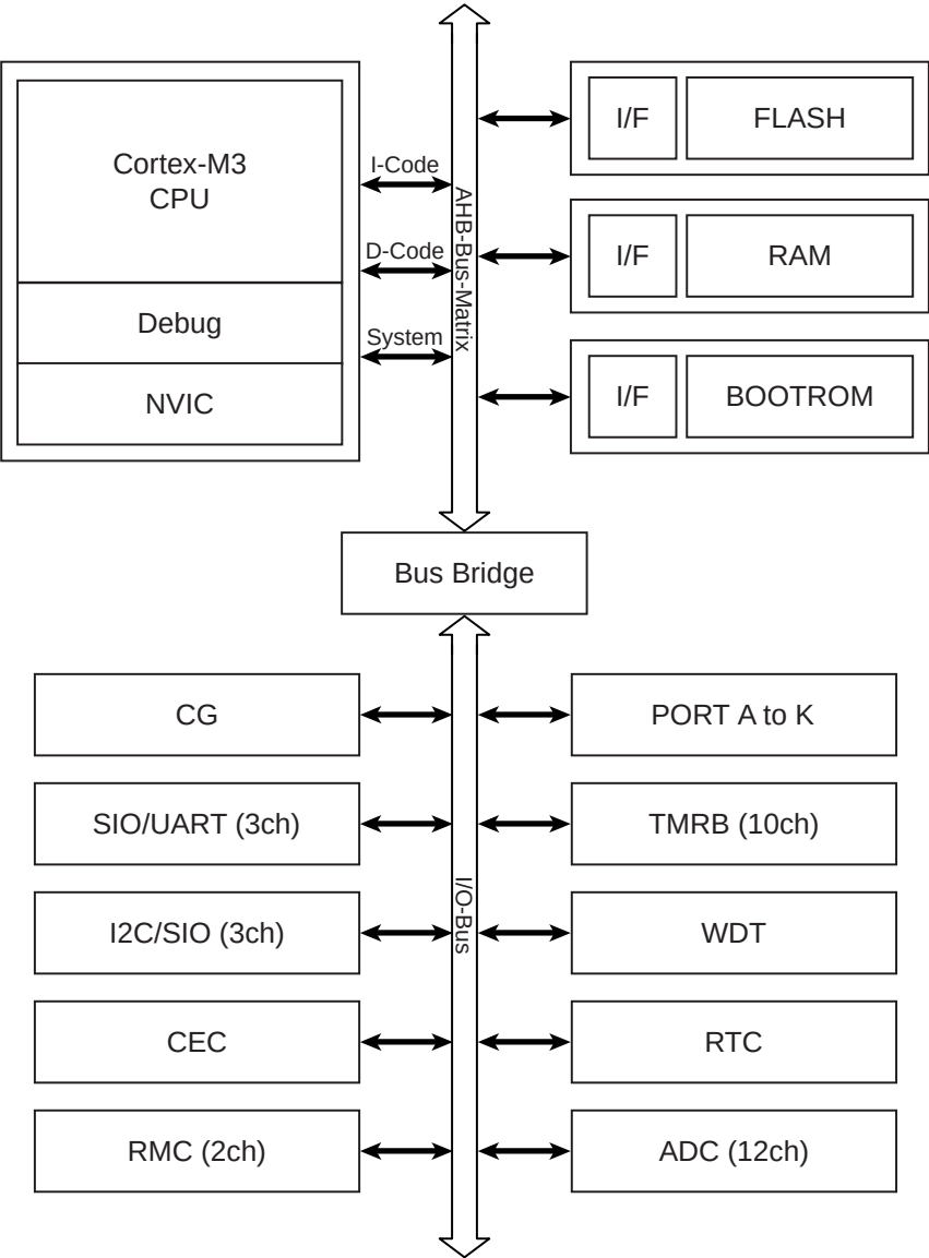
Figure 1-1 TMPM330FDFG/FYFG/FWFGBlock Diagram
