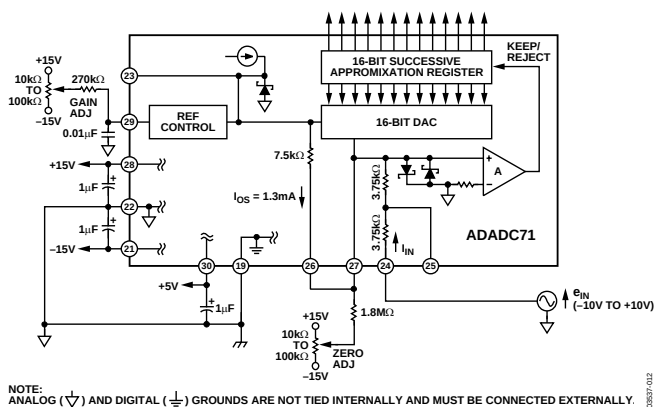
Figure 12. Analog and Power Connections for Bipolar -10\text{ V} to +10\text{ V} Input Range
